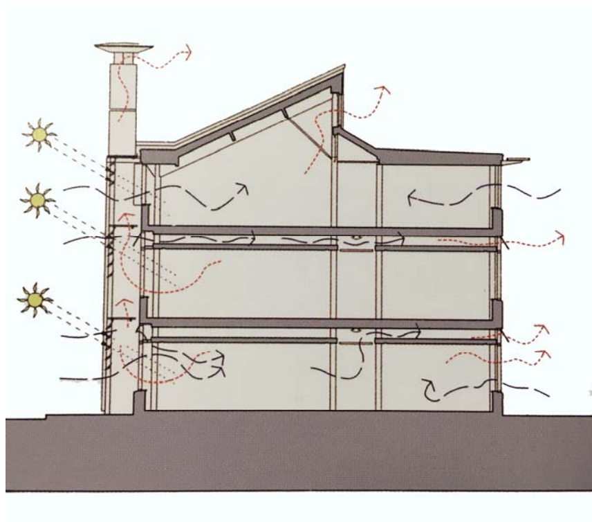
Figure 35: BRE office building section; showing cross and stack assisted ventilation paths. (Feilden Clegg Architects)
