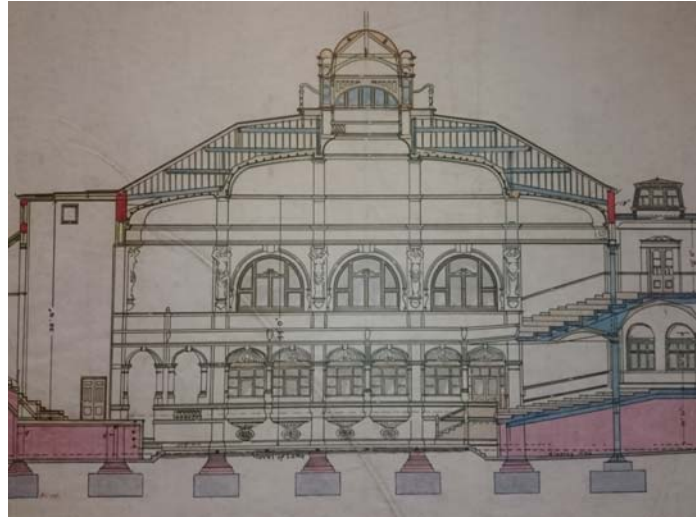
Figure 40: Kursaal, section, Harrogate UK –(F. Mitcham Architect)
