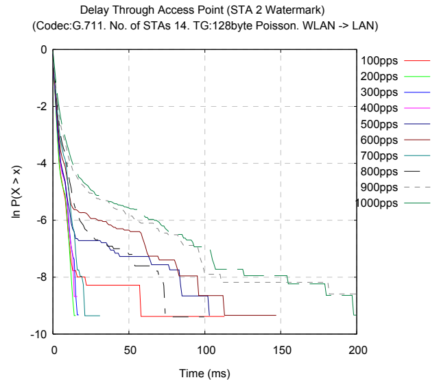
Figure 5.43(b): STA 2 Watermark plots.
