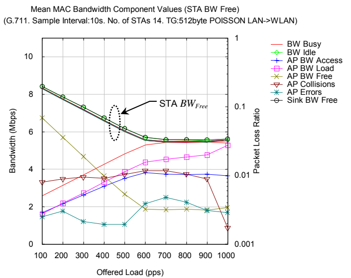
Figure 5.47(a): STAs dropped after 600 pps. Figure 5.47(b): STA BW_{Free} \approx 5.55 Mbps at 600 pps.
