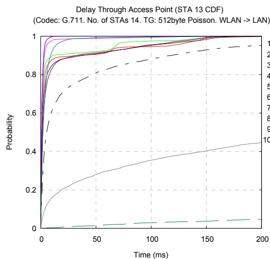
Figure 5.34(a): STA13 CDF of AP transit delay.
