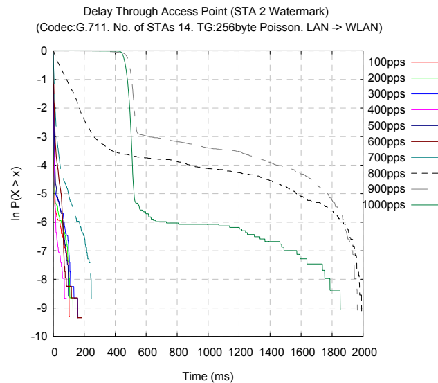
Figure 5.65(b): STA 2 Watermark plots.
