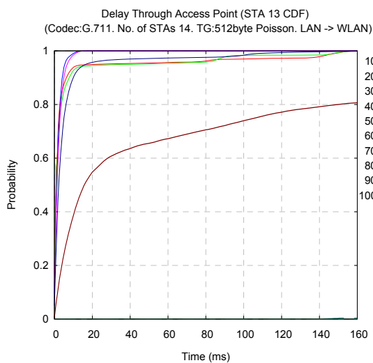
Figure 5.58(a): STA 13 CDF of AP transit times.
