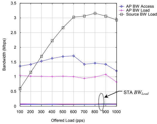
Mean MAC Bandwidth Component Values (STA BW Load) (G.711. Sample Interval:10s. No. of STAs 14. TG:512 byte POISSON WLAN->LAN)
