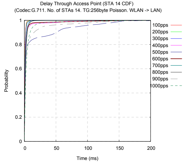
Figure 5.36(b): STA14 CDF of AP transit delay.
