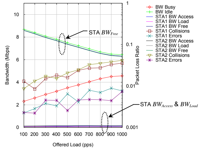
Figure 5.54(b): Comparison of STA1 & STA2.
