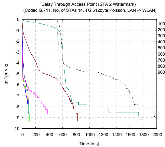
Figure 5.63(b): STA 2 Watermark plots.
