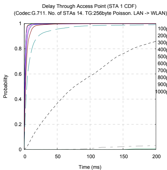
Figure 5.59(a): STA 1 CDF of AP delay.
