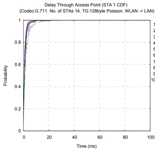
Figure 5.37(a): STA1 CDF AP transit delay.
