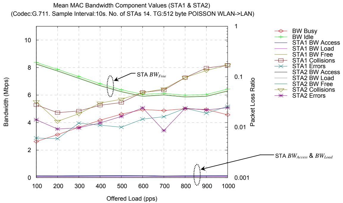
Figure 5.24: MAC BW values and PLR for a conversation pair.
