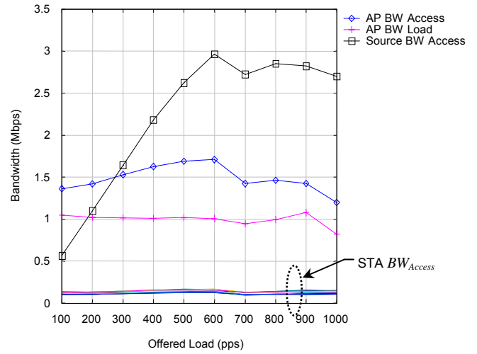
Mean MAC Bandwidth Component Values (STA BW Access) (G.711. Sample Interval:10s. No. of STAs 14. TG:512 byte POISSON WLAN->LAN)
