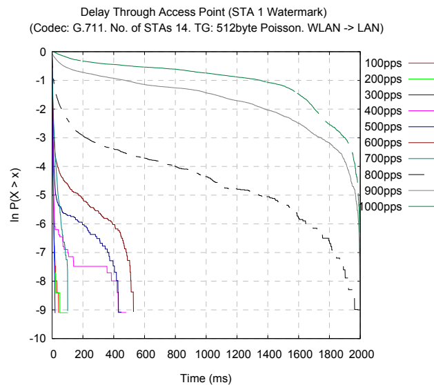
Figure 5.39(a): STA 1 Watermark plots.
