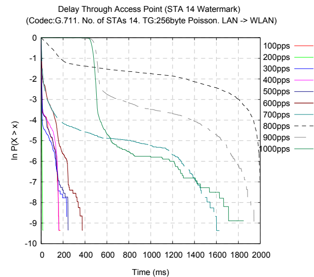
Figure 5.66(b): STA 14 Watermark plots.
