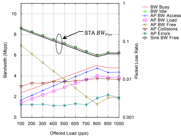
Mean MAC Bandwidth Component Values (STA BW Free) (G.711. Sample Interval:10s. No. of STAs 14. TG:256byte POISSON LAN->WLAN)
