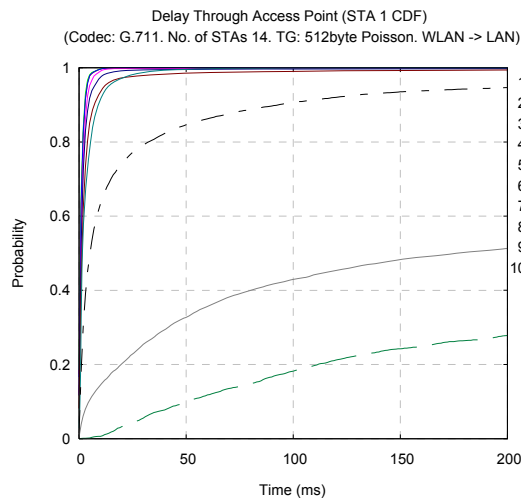
Figure 5.33(a): STA1 CDF of AP transit delay.
