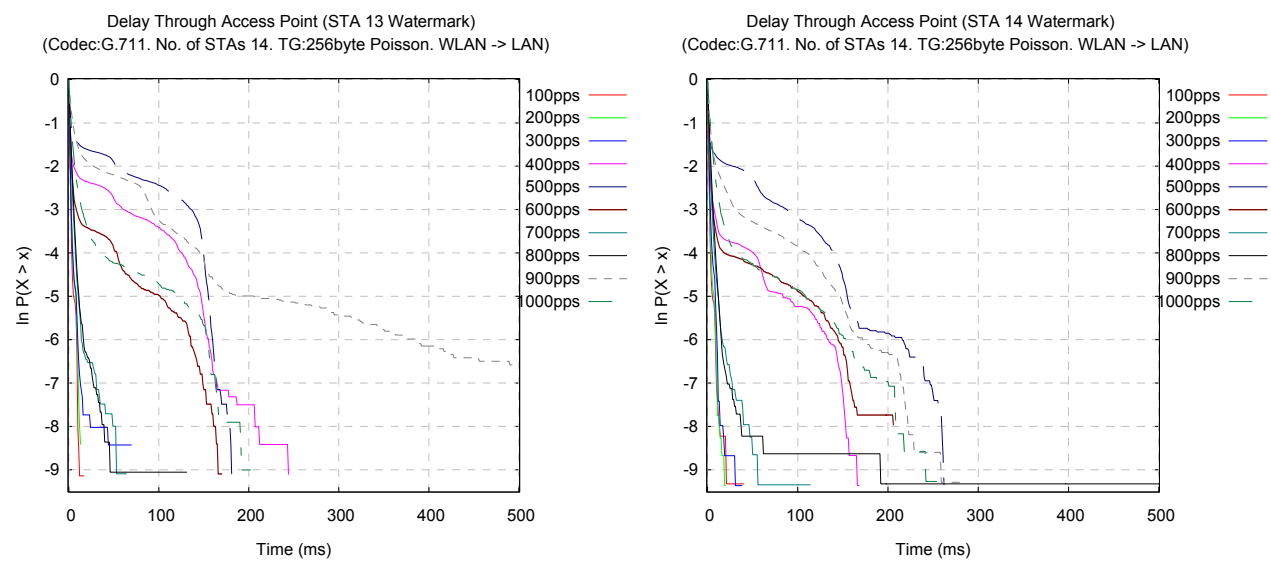
Figure 5.42(a): STA 13 Watermark plots.
