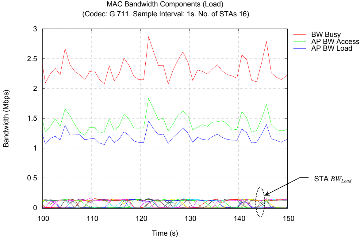
Figure 5.11: STA BW_{Load} for 16 STA test.
