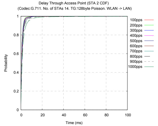
Figure 5.37(b): STA2 CDF AP transit delay.
