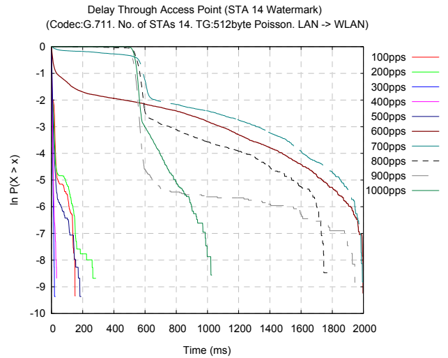
Figure 5.64(b): STA 14 Watermark plots.
