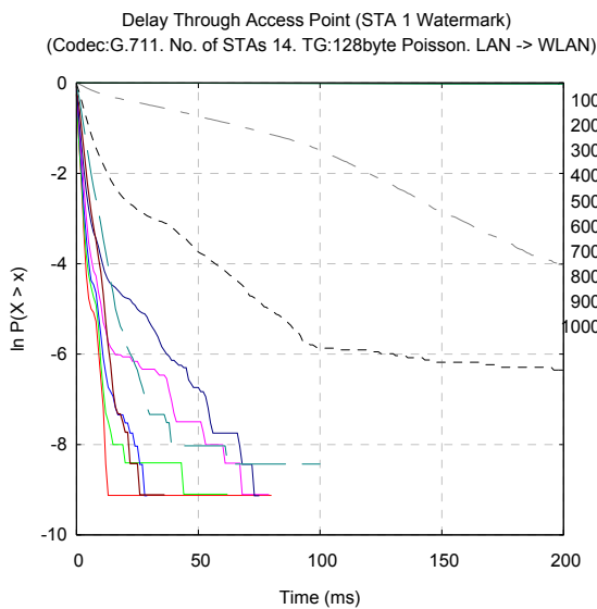
Figure 5.67(a): STA 1 Watermark plots.
