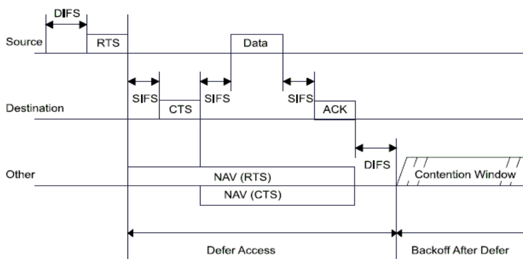
Figure 2.8: RTS/CTS/Data/ACK and NAV setting [10].
