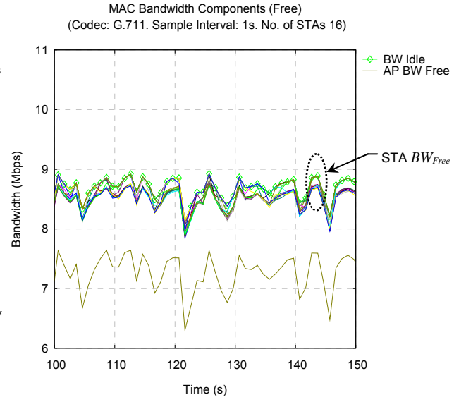
Figure 5.12 (b): BW_{Free} for 16 STA test.
