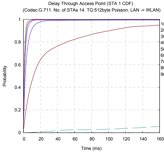
Figure 5.57(a): STA 1 CDF for increased TG rate.
