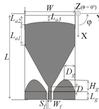
Figure 1. Monopole antenna.
