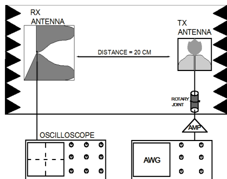
Figure 1: Time domain measurement setup.
