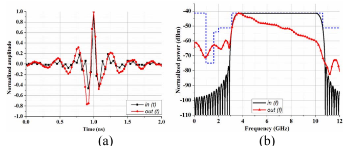
Figure 2: (a) Digitized SRRC waveform in(t) & amplified AWG output signal out(t) and (b) their respective normalized power spectrum density.
