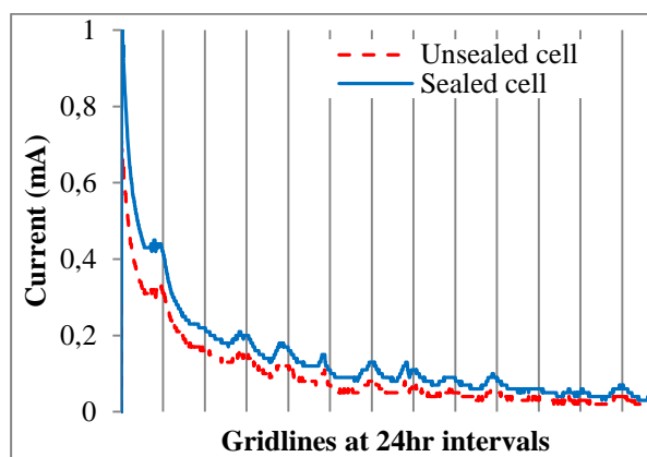
Figure 8. Discharge current through a 10\Omega resistor for a sealed and unsealed battery.
