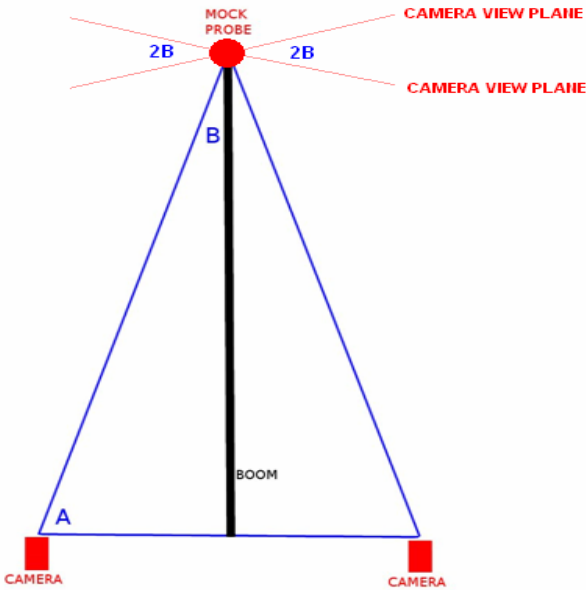
Figure 8: Principle of operation for camera system
