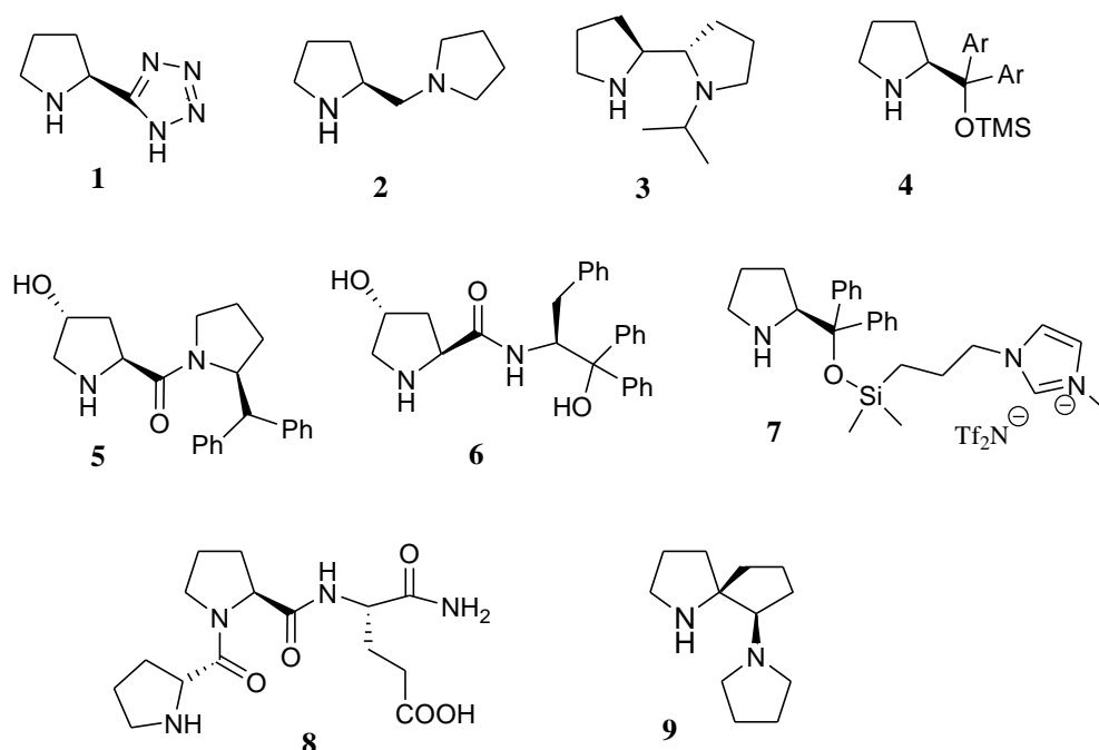
Figure 1. Proline and 4-hydroxyproline derived organocatalysts. 1-6
