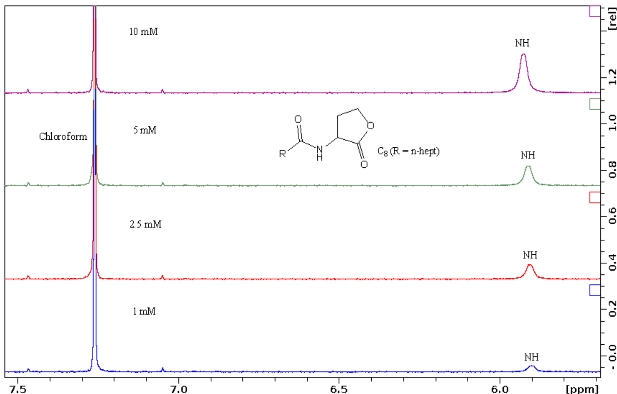
Figure 1. Stacked 1 H NMR spectra of C 8 AHL at 1-10 mM, in CDCl 3 at 7 days
