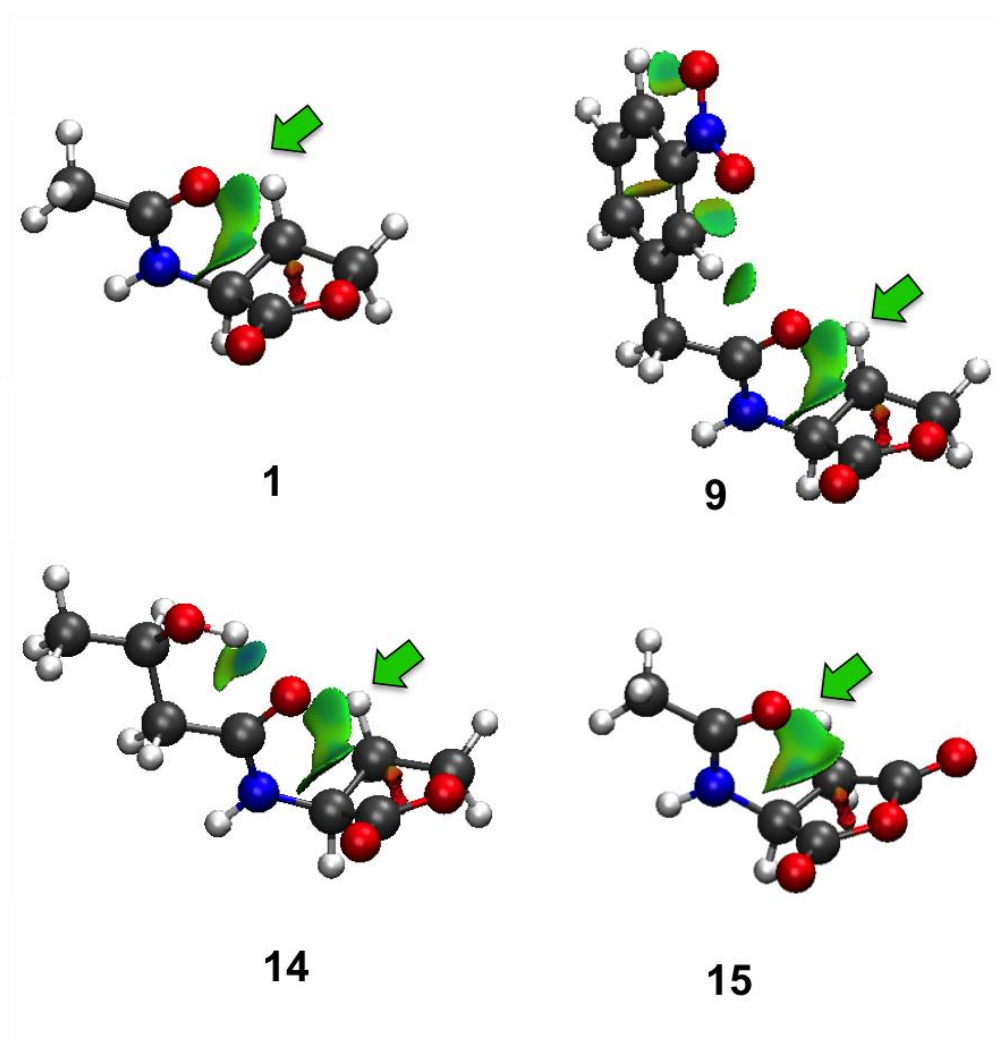
Figure 5. Non-covalent interaction (NCI) plots for the np conformations of 1 , 9 , 14 and 15 , in acetonitrile. Green areas correspond to \lambda_2 \approx 0 (weak). \lambda_2 is one of the three eigenvalues of the electron density Hessian with \lambda_1 \leq \lambda_2 \leq \lambda_3 . 12
