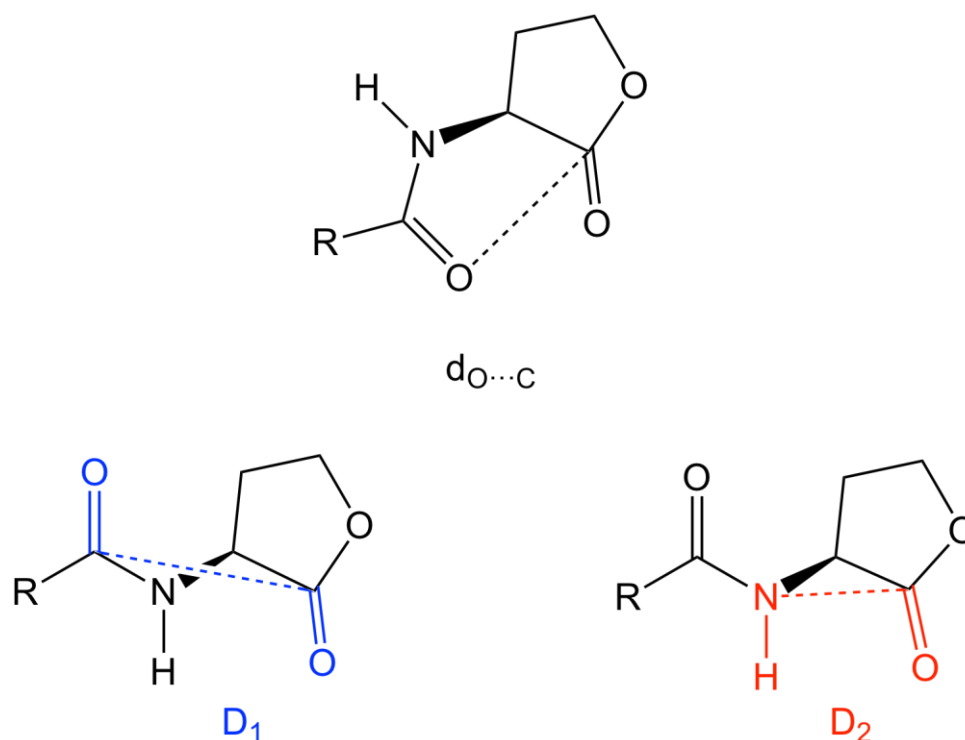
Figure 4. Distance d_{O...C} and dihedral angles ( D_1 and D_2 ) analysed for the X and np conformations, for compounds 1-15
