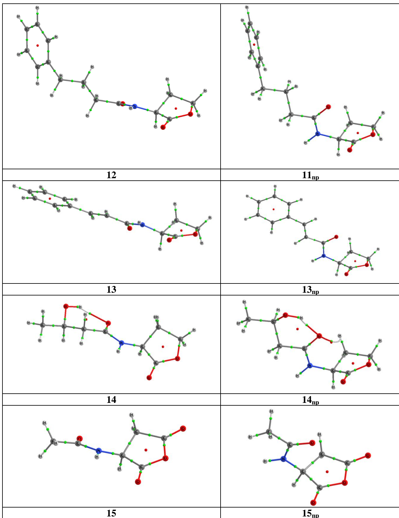
Figure S1. Molecular graphs for all the X and np compounds studied at the M06-2X/6-311++G(d,p) computational level using PCM (acetonitrile).
