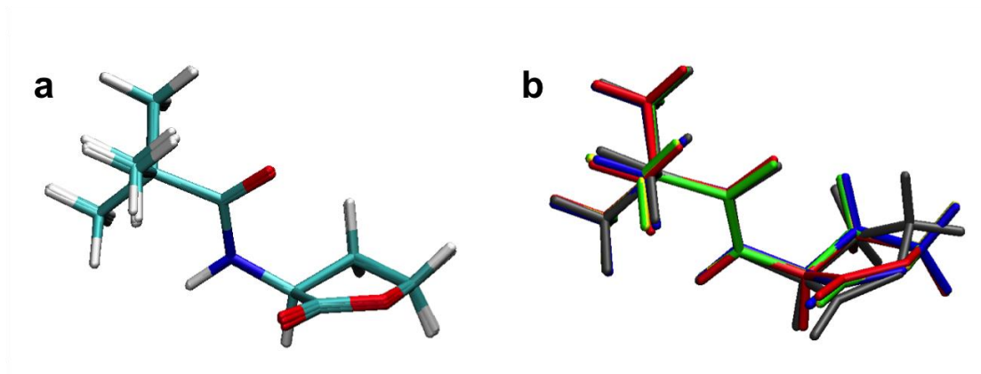
Figure 3. a) Overlap between the np conformations of 6 at MP2, B3LYP, B3LYP-D3, M06-2X and WB97XD levels. b) Overlap between np conformations of 6 (from reference 14 (in grey)) in gas phase and calculated in the present work in gas phase (blue), chloroform (red), acetonitrile (yellow) and water (green) solvent models.
