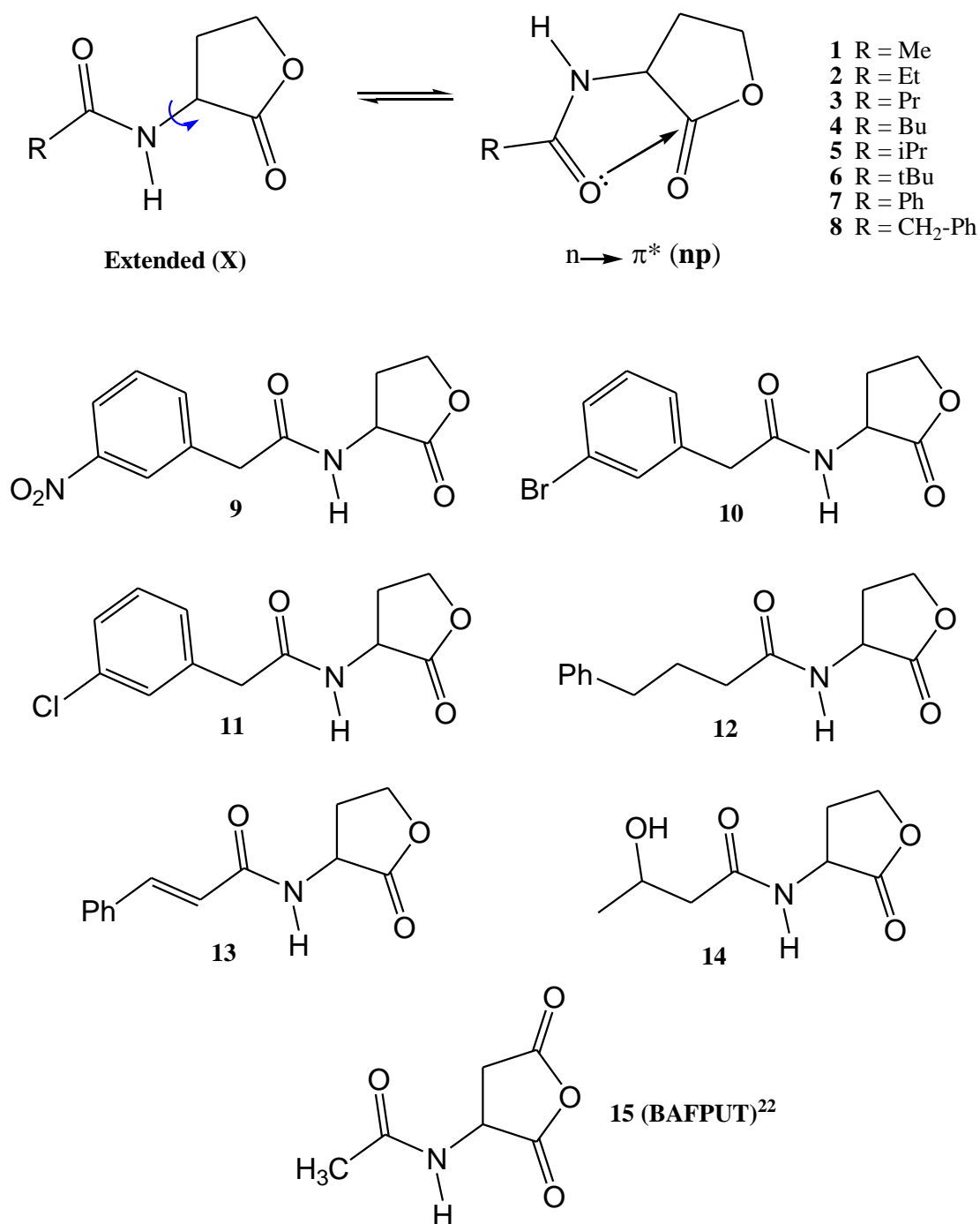
Figure 2. Compounds included in this study. The extended conformation is denoted X , while np indicates the conformation with an n \rightarrow \pi^* interaction
