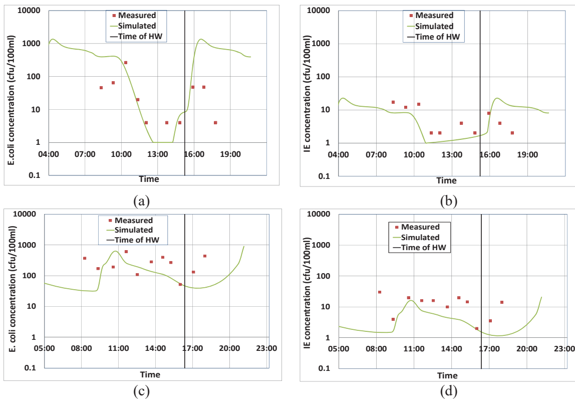
Fig. 5 Observed and simulated E.coli and I.E at Location O on the 5 th September 2012 ((a) and (b)) and at location L on the 23 rd August 2012 ((c) and (d))
