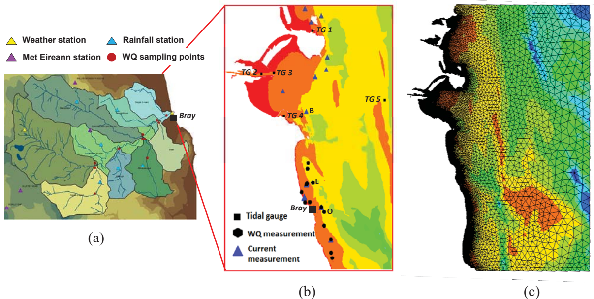
Fig. 2 Data collection stations in the River Dargle catchment (a) and in Bray coastal zone (b). The model mesh is shown in (c).
