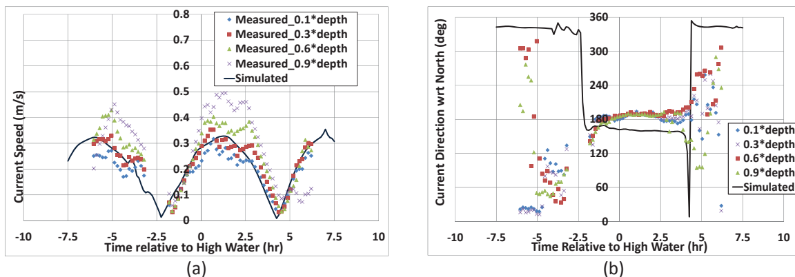
Fig. 4 Comparison of simulated depth averaged current velocity (a) and direction (b) with measured values at 10%, 30%, 60% and 90% depths in the water column at location B
