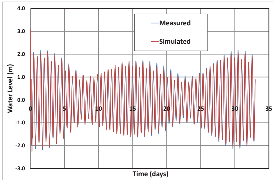
Fig. 3 Observed and simulated tide levels at TG 4 from 29 th September to 31 st October, 1989
