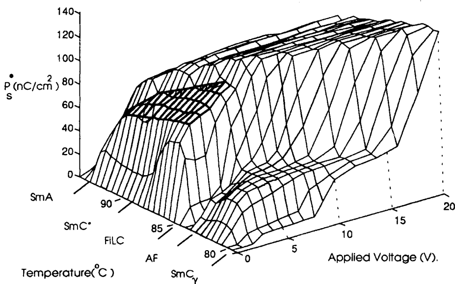
FIGURE 1 Spontaneous polarization P_s^* ( \text{nC}/\text{cm}^2 ) versus Temperature ( ^\circ\text{C} ) and Applied Voltage (V). The region in bold lines is proposed to be a FiLC phase.
