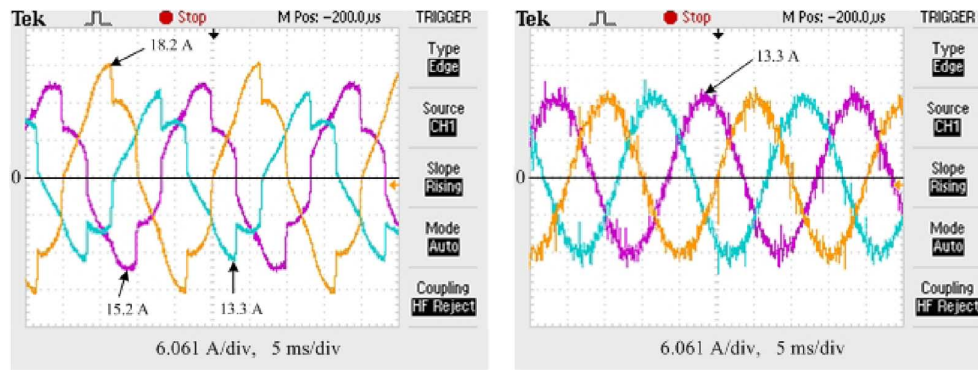
Fig. 9. Load unbalance. (a) Load currents. (b) Supply currents (THD = 4.5%).
