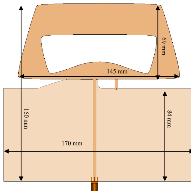
Figure 1. Geometry and dimensions of the printed monopole antenna.
