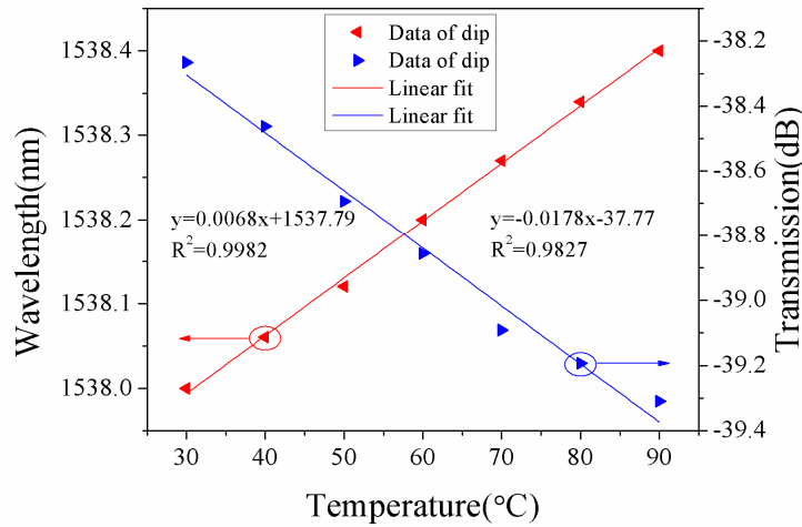
Fig. 11. Dip shift as a function of temperature. The red line represents wavelength-temperature fitting, the blue line represent intensity-temperature fitting.
