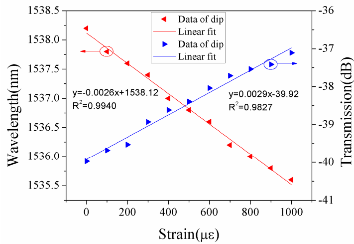
Fig. 7. Dip shift as a function of strain. The red line represents wavelength-strain fitting, the blue line represents intensity-strain fitting.
