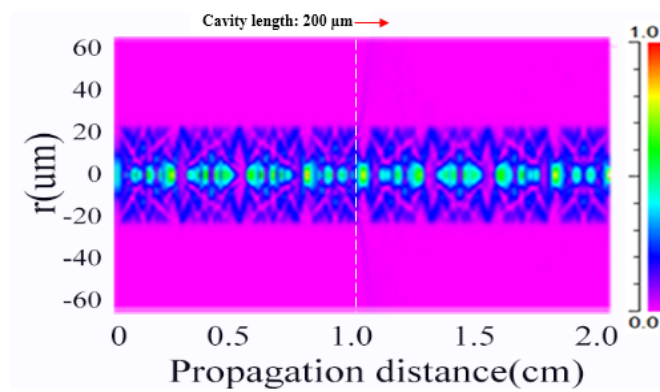
Fig. 4. Simulated optical field intensity distribution within an SGMS fibre structure at a wavelength of 1550 nm using a BPM.
