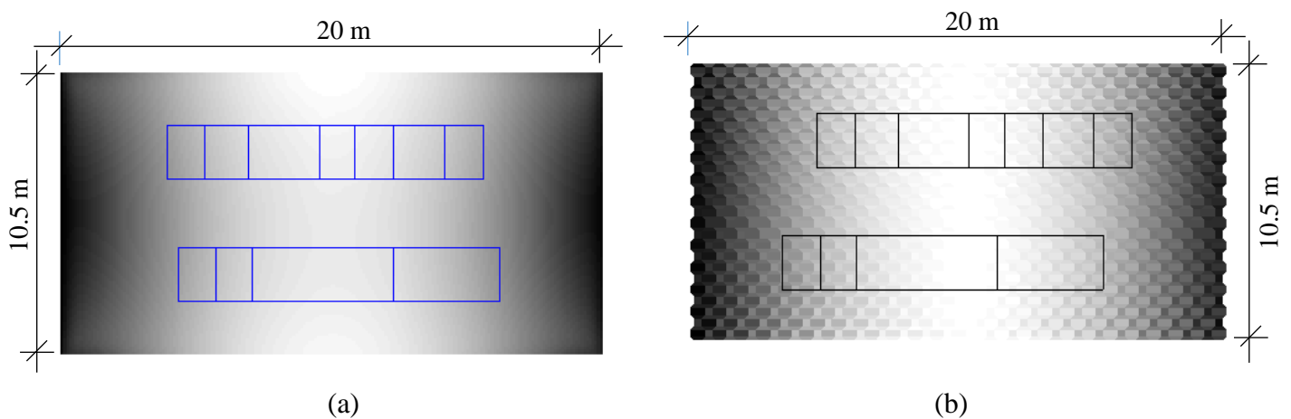
Figure 6 Bending moment contours for critical case (light color indicates higher moment): (a) 2D linear analysis; (b) 2D nonlinear analysis
