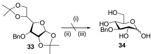
Scheme 2-24 Reagents and Conditions: (i) 1M HCl:THF (1:1) rt. 30 (ii) MeOH, Cat I 2 , rt. 30 (iii) 60% aq. AcOH rt. 31
