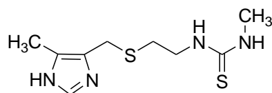
Figure 1-4 Metiamide.
