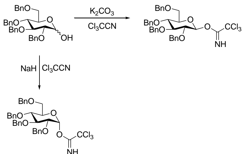
Figure 2-8 Trichloroacetimidate formation. 11
