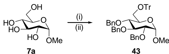
Scheme 3-3 Reagents and Conditions: (i) Py anhydr., \text{TrCl} , imidazole, 40^\circ\text{C} . (ii) DMF anhydr., \text{NaH} , \text{BnBr} , rt. (37% yield over 2 steps). 16
