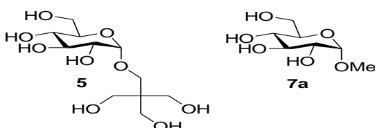
Figure 2-10 (5) \alpha -Glycoside (7a) Methyl \alpha -D-glucopyranoside.
