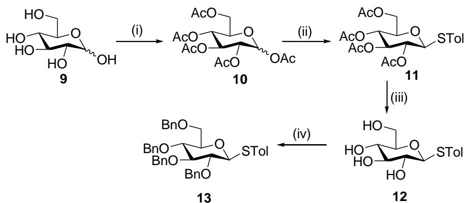
Scheme 2-13 Reagents and Conditions: (i) Ac 2 O, Py, rt. (41% yield) (ii) p -Thiocresol, CH 2 Cl 2 , 0°C, BF 3 ·Et 2 O. (15% yield) (iii) Na, MeOH, rt. (iv) DMF anhydr., BnBr, 0°C, NaH, rt. (53% yield over 2 steps) 24
