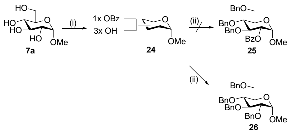
Scheme 2-20 Reagents and Conditions: Dioxane, \text{Bu}_2\text{Sn}(\text{OMe})_2 , \text{BzCl} , rt. (23% yield) 23 (ii) DMF anhydr., \text{BnBr} , 0^\circ\text{C} , then \text{NaH} , rt. (79% yield)
