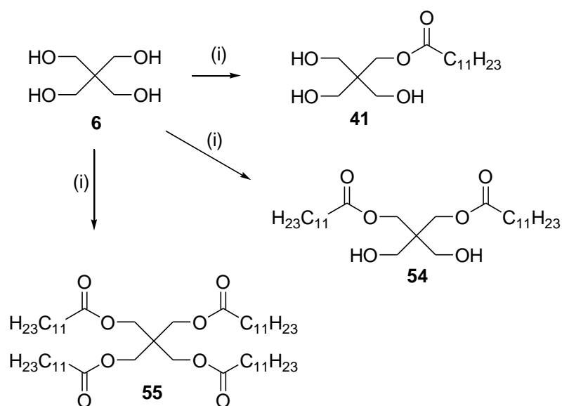
Scheme 3-9 Reagents and Conditions: (i) Py anhydr., DMAP, Lauroyl Cl, rt. ( 41 : 14% yield, 54 : 29% yield, 55 : 6 % yield)
