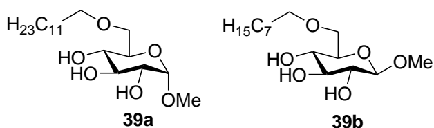
Figure 3-6 Methyl 6- O -dodecanyl- \alpha -D-glucopyranoside ( 39a ) and methyl 6- O -dodecanyl- \beta -D-glucopyranoside ( 39b ).
