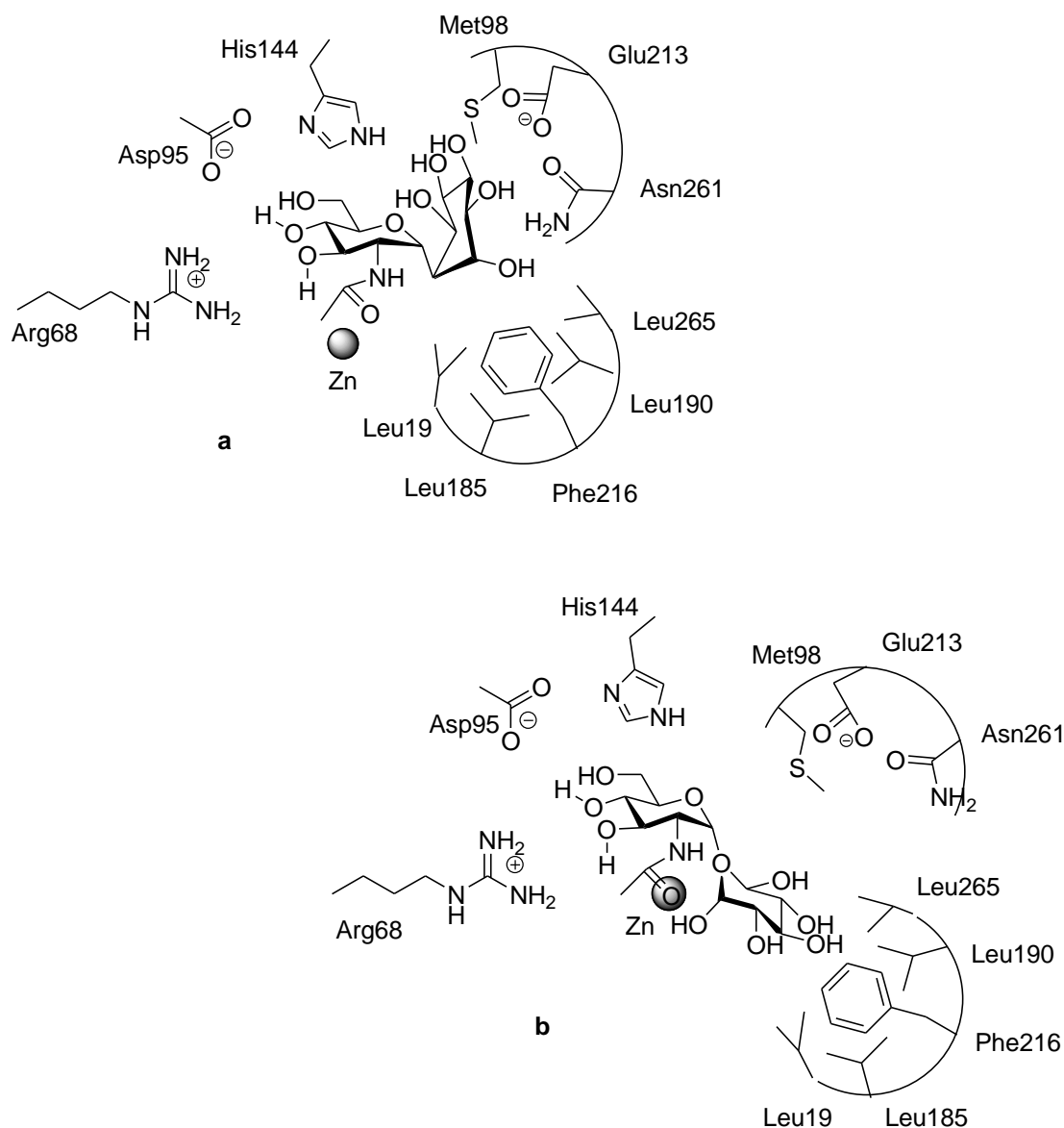
Figure 1-18 Proposed substrate-binding mode of GlcNAc-Ins in mshB based on molecular modelling of BOG molecule. 63
