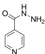
Figure 1-12 Structure of Isoniazid. 56
