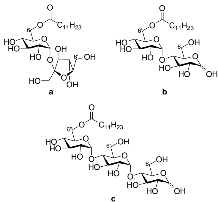
Figure 1-29 6- O -lauroylsucrose (a), 6'- O -lauroylmaltose (b) and 6''- O -lauroylmaltotriose (c). 132
