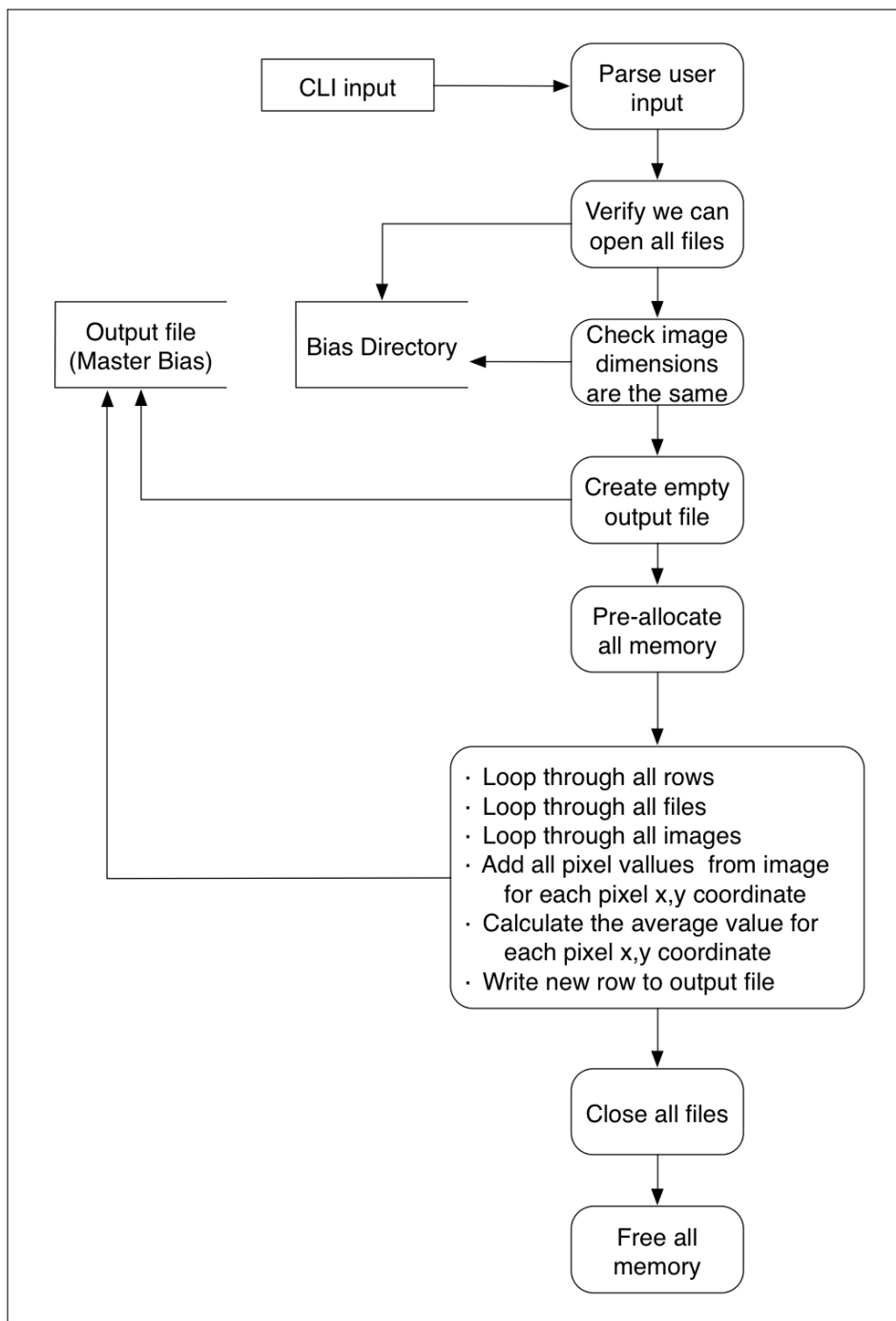
Figure B.2: FEBRUUS: The GMB.c program flowchart
