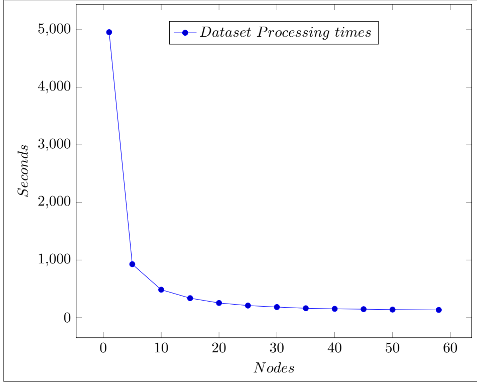
Figure 4.10: ACN5: Data cleaning for increasing numbers of ACN nodes in seconds. Includes compression time of 109 seconds and upload time of 200 seconds
