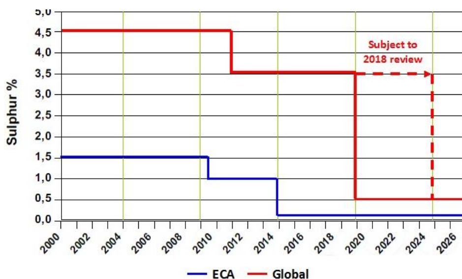
Figure A6.2: Fuel Oil Sulphur limits
