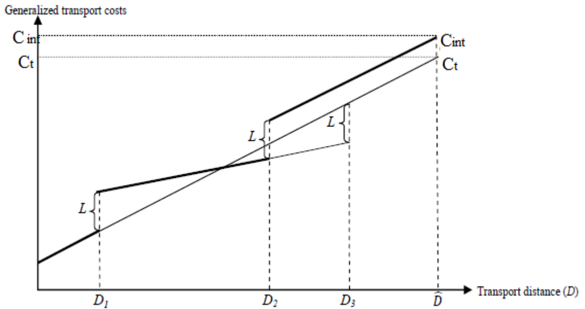
Figure 5.5 Relationship between generalized transport costs over transport distances Source: Several; Janic 2007; Hanssen et al 2012.
