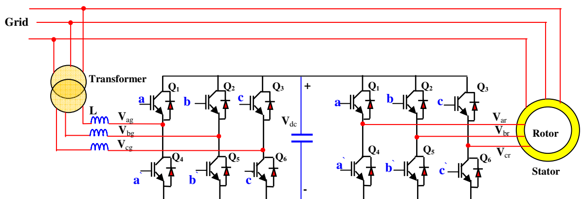
Figure 6.11 IGBT transistors on rotor side and grid side converters
