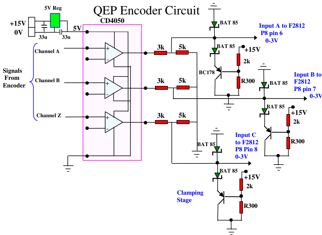
Figure 8.19 Incremental shaft encoder interface circuit QEP
