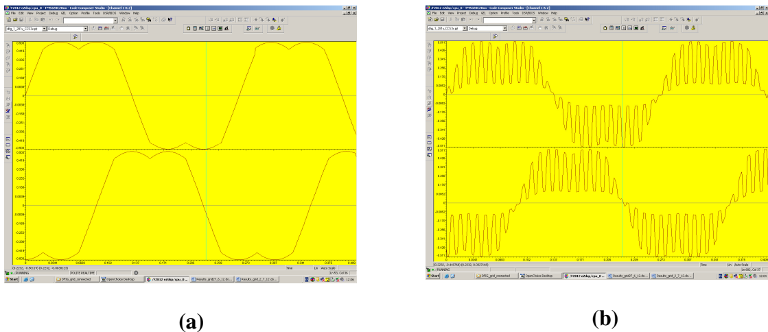
Figure 9.10 Output of space vector generator in software: (a) before PIR compensation and (b) with PIR compensation
