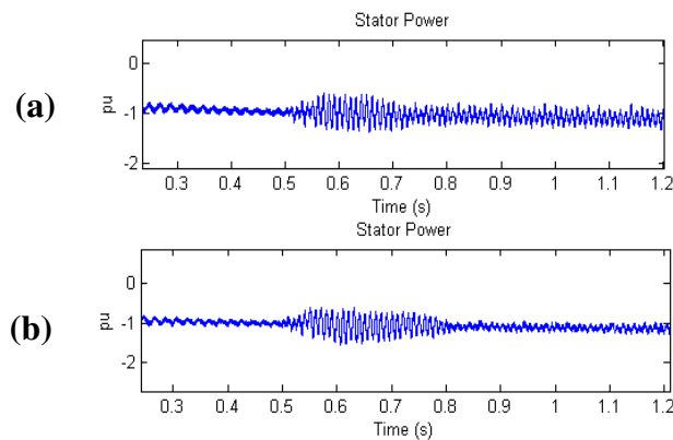
Figure 7.27 Stator Power ((a)-Standard Control- (b) PIR Compensation)
