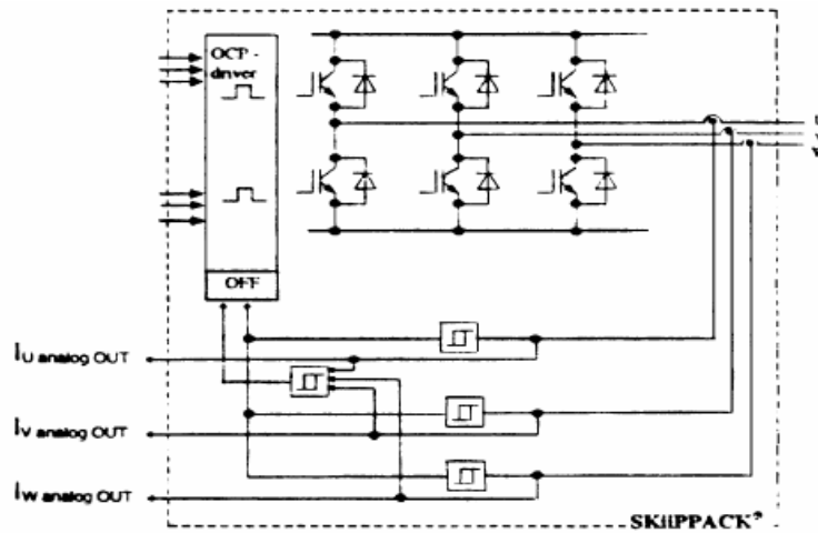
Figure 8.6 IGBT over current protection
