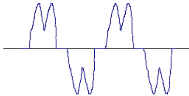
Figure 2.6 Typical line current waveform of a three-phase diode rectifier system when the supply system is balanced
