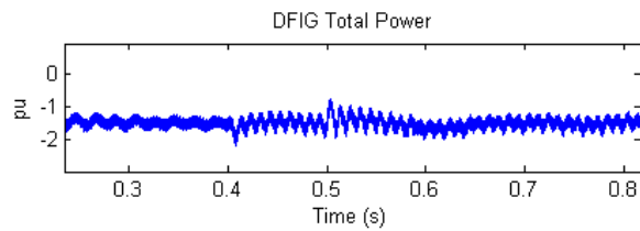
Figure 7.17 DFIG total power – no grid side compensation
