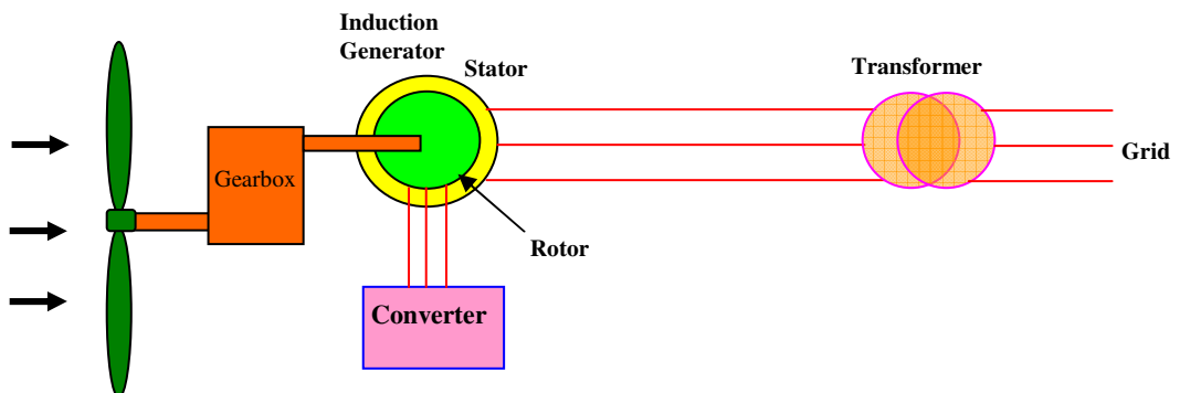
(c) Variable Speed: Variation of Rotor Resistance with with Power Converter
