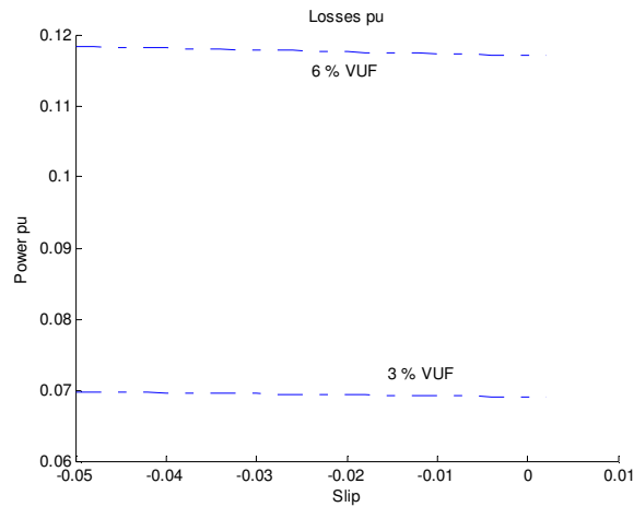
Figure 4.25 Losses as a result of applied voltage unbalance to an 800 kW induction machine
