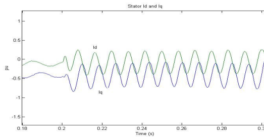
Figure 6.25 Stator i_d and i_q currents
