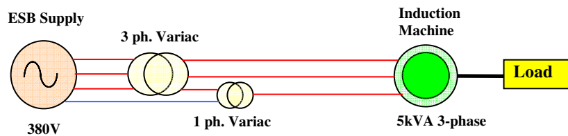
Figure 4.23 Induction machine circuit for voltage unbalance testing
