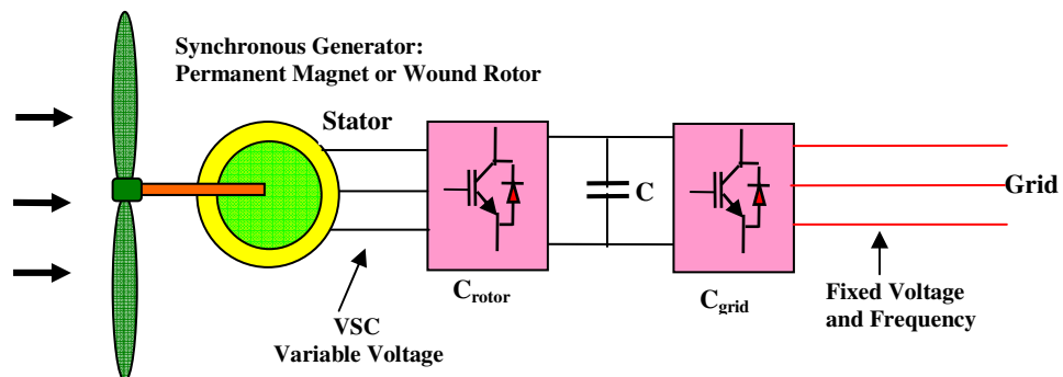
(b) Direct-drive generator with power converter
