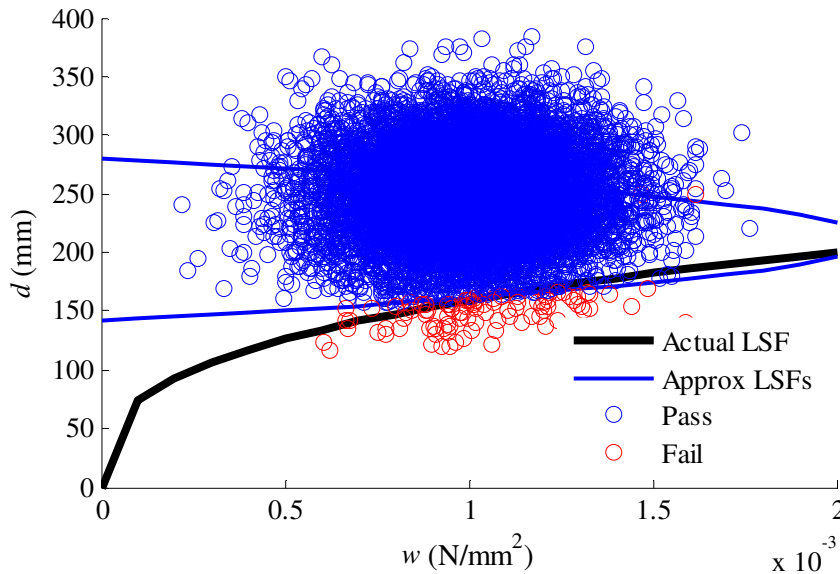
Figure 5.8: Correct importance sampling plot.
