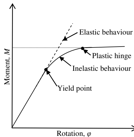
Figure 4.1: Moment rotation curve (adapted from Becker, 2004)
