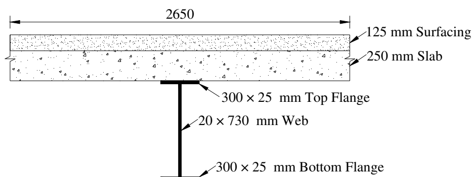
Figure 6.2: Composite cross section used for each bridge studied.
