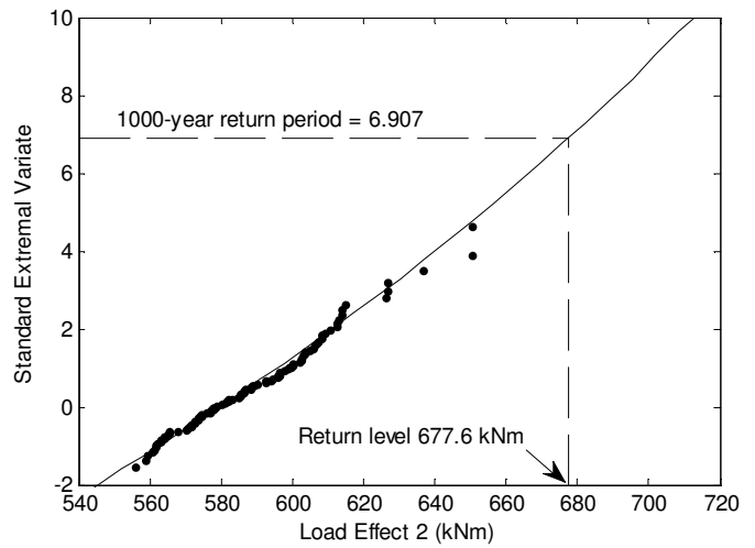
Figure 7. Sample extrapolation to 1000-year return period for Load Effect 2.
