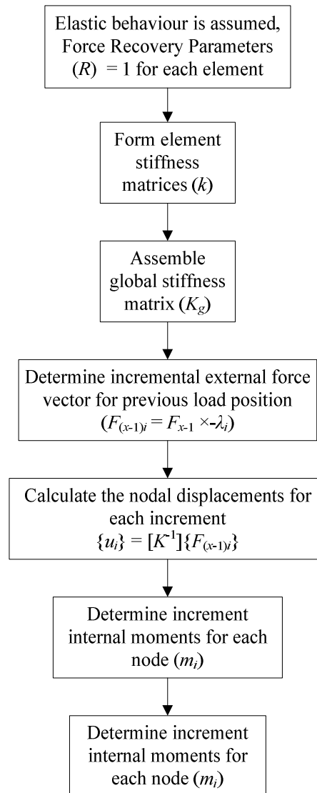
Figure 7.4: Unloading process
