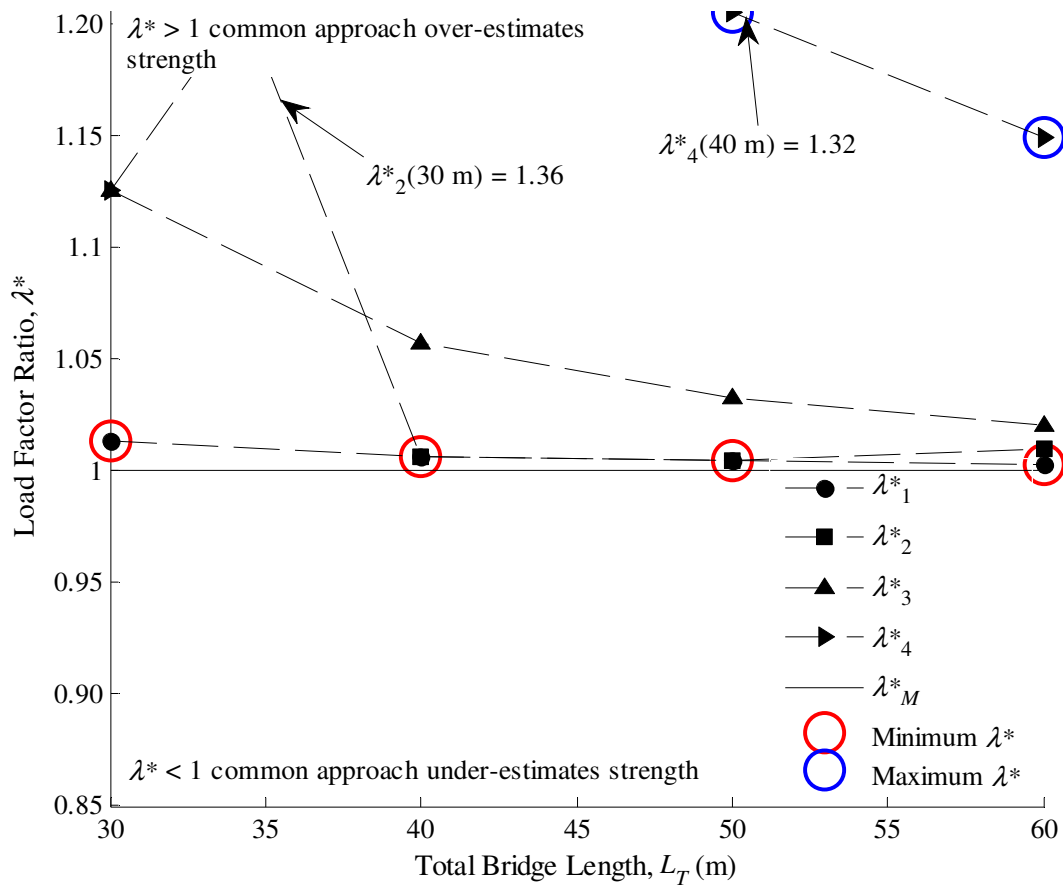
Figure A1.18:AS2-6.0 (two axles 6.0 m apart)
