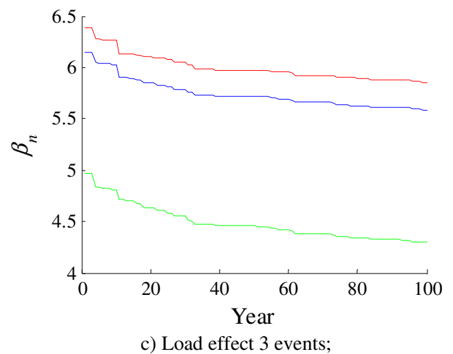
Figure A5.14: Three-span 40 bridge reliability indices cumulative reliability indices.
