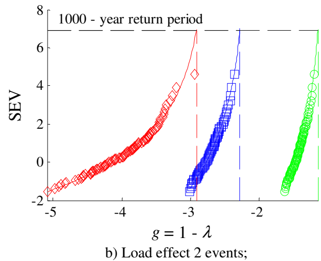
Figure A2.6: Two-span 50 bridge limit state extrapolation.
