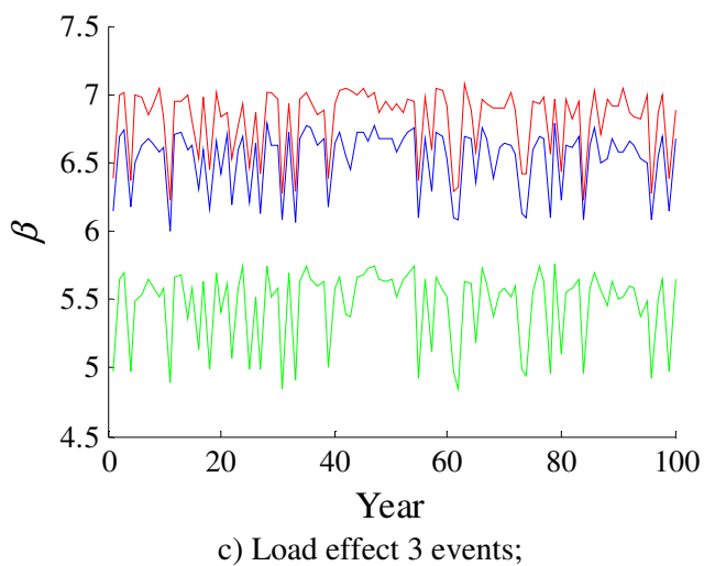
Figure A5.13: Three-span 40 bridge reliability indices.
