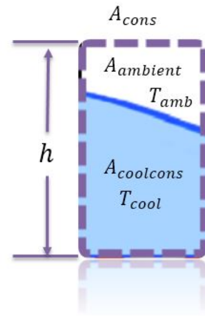
Fig. 5. Mixing concentrations of cooling supply air and hot ambient air
