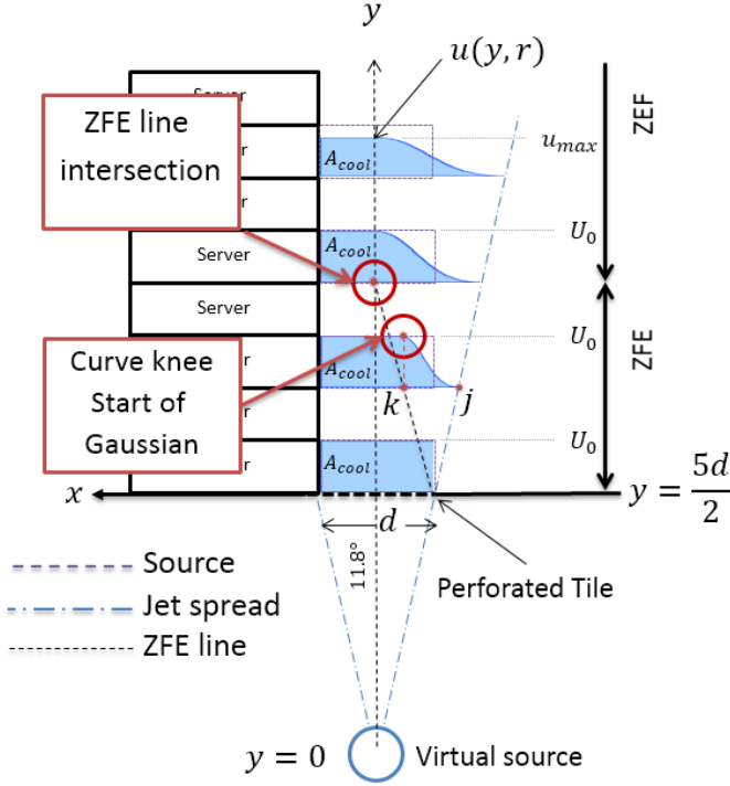
Fig. 3. Round Free Turbulent Jet - the velocity profile is simplified. A ZFE line is drawn from the edge of the perforated tile flow at U_0 to the centre of the curve at u_{max} at the point along y where the ZFE begins. The intersection of the ZFE line with the any of the sample lines determines the knee of the curve (start of the Gaussian curve).
