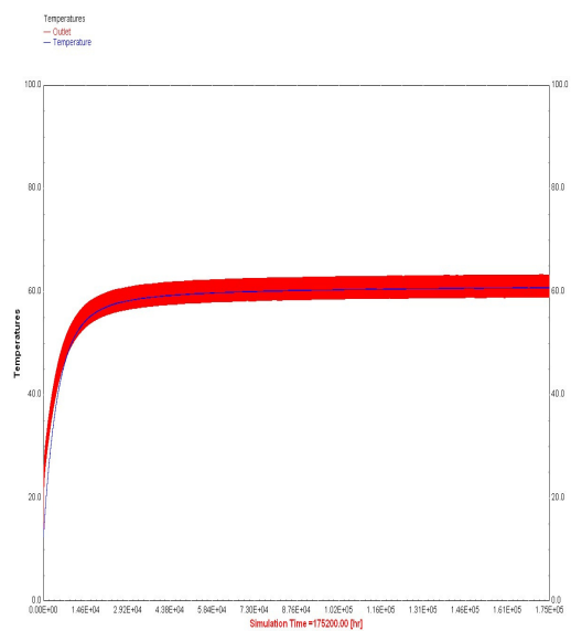
Figure 2: 20 year operation of 40no. 50 meter deep boreholes
