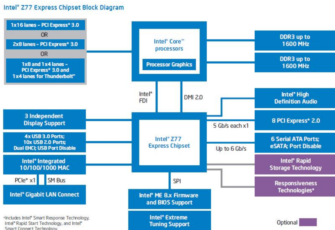
Figure: Intel z77 Express Chipset Block Diagram
