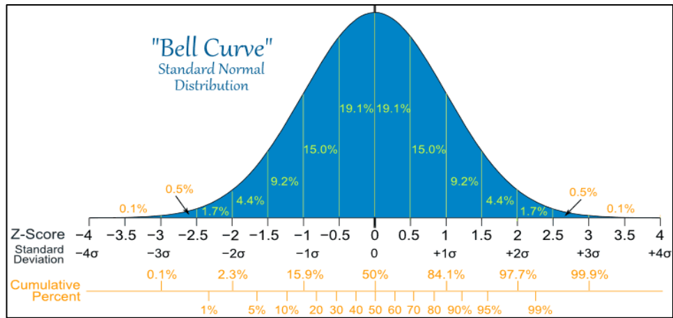
Figure 3.3: Bell Curve
