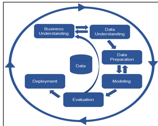
Figure 3.1: CRISP-DM framework
