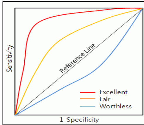
Figure 3.7: ROC chart
