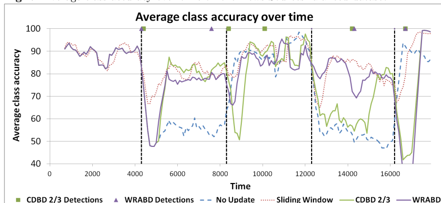
Fig. 8 Average class accuracy over time on the Reuters dataset
