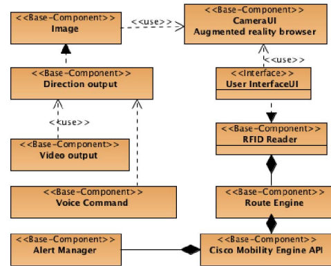
Fig. 5. IWayFinder Core-Classes Structure
