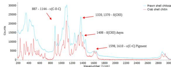
Fig 10: Overlaid Raman Spectra of Crab Shell Chitin and Shrimp Shell Chitosan Standard.
