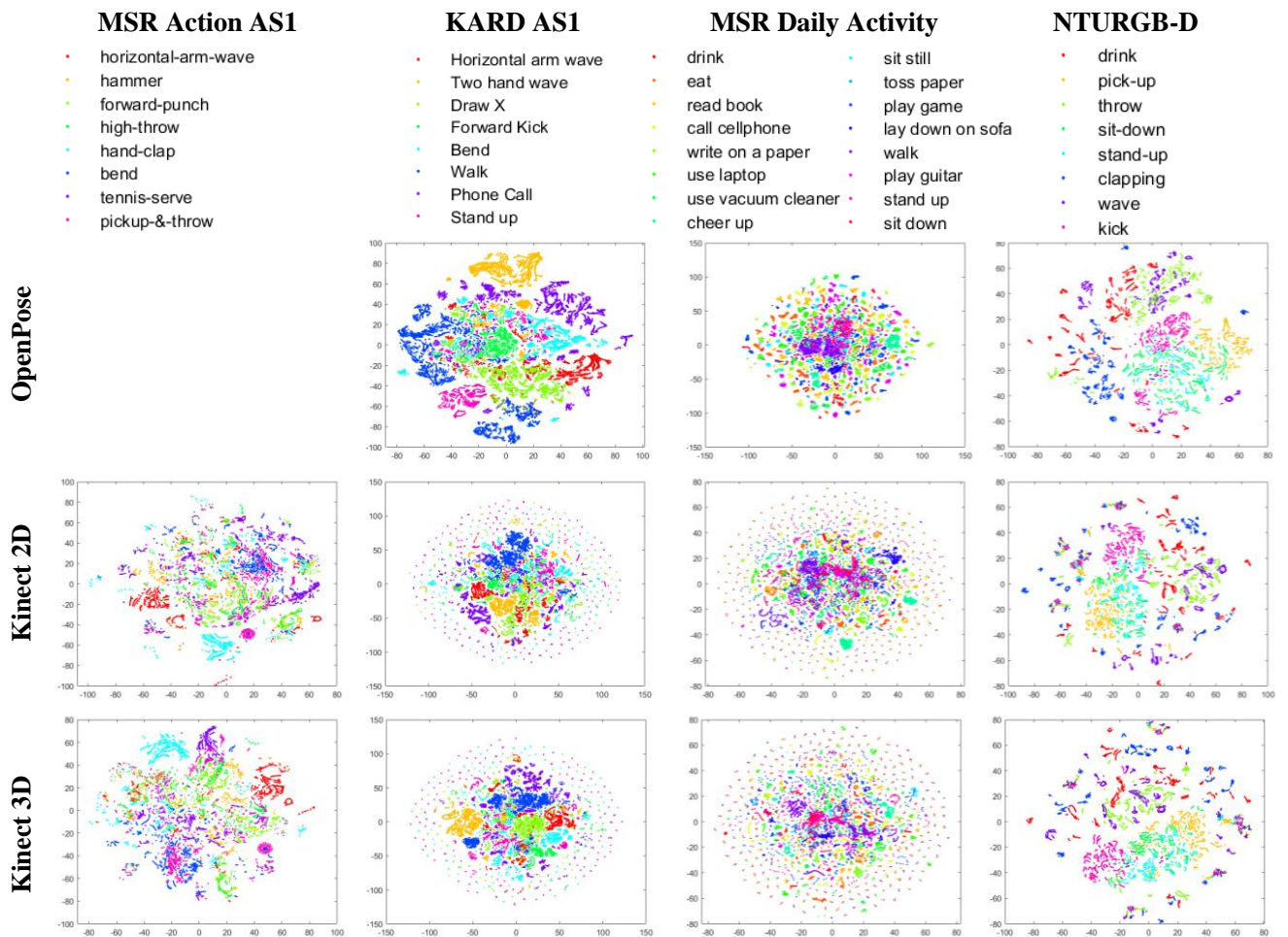
Figure 3: t-SNE plots showing similar patterns for each dataset demonstrate that data collected from the different sources provides similar information for classifying activity. Less ‘ball’ scatter in the KARD and MSR Daily Activity OpenPose plots is as a result of fewer frames (best viewed in colour)
