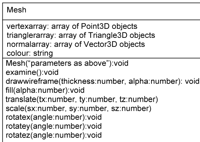
Figure 15: Class diagram for the Mesh class
