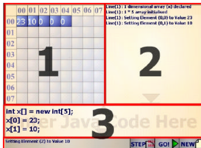
Area 1. Displays an 8 * 8 grid of the created array with the values stored in each element.
