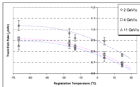
Figure 6: Registration temperature effect using relativistic gold at three different energies
