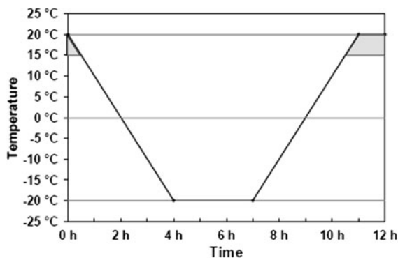
Fig. 8 Freeze thaw cycle for RILEM test [19]
