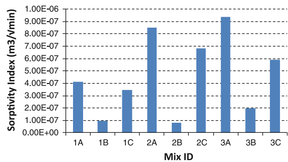
Fig. 13 Sorptivity indices of the various mixes
