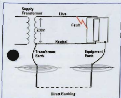
Figure 3 — A direct earthing system
