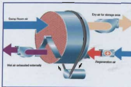
Figure 1. Typical Desiccant Wheel dehumidifier arrangement (Munters Dessicant Rotor).
