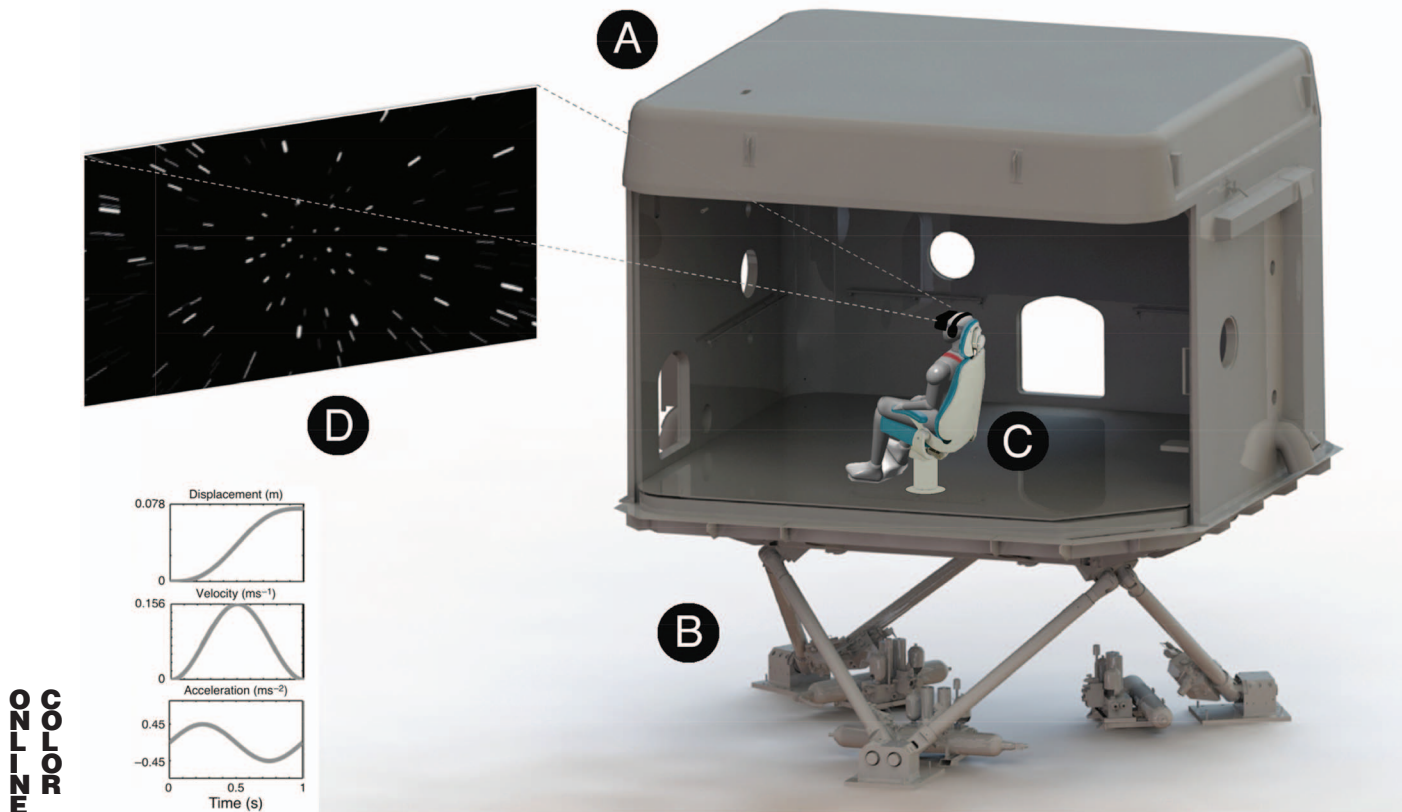
FIGURE 1 Figure 1. Depiction of the lab used for this study (A) located at the Toronto Rehabilitation Institute. This lab consists of an 8m 3 fiberglass cabin with a steel floor. The lab was mounted to a 6-degree-of-freedom hydraulic motion platform, (B) which provided vestibular cues to heading via passive translation. Participants were seated in a chair that was bolted to the floor (C), and they wore an Oculus Rift stereoscopic head-mounted display (HMD) and noise isolating headphones. The HMD provided optic flow via stereoscopic imagery of an expanding starfield (D). Inset are the characteristics of the visual and vestibular motion profiles. See the online article for the color version of this figure.
