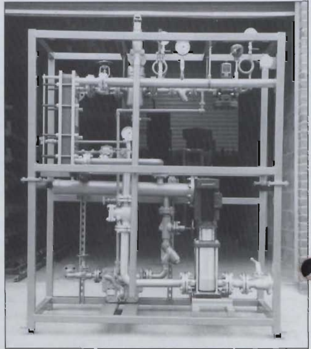
Europak heating and cooling packaged heating transfer unit from Eurofluid Handling Systems.
