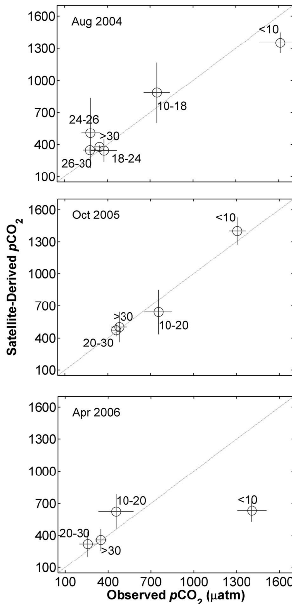
Figure 7. Match ups between satellite-derived and in situ p\text{CO}_2 binned by salinity range showed generally good agreement, with the exception of the <10 salinity data in August 2004 and April 2006, the 24–26 salinity range data during August 2004, and the 10–20 salinity range data during April 2006. Greater variability in the plume region and temporal offsets between the times for acquiring in situ and satellite data contributed to the differences between match ups at lower salinities.
