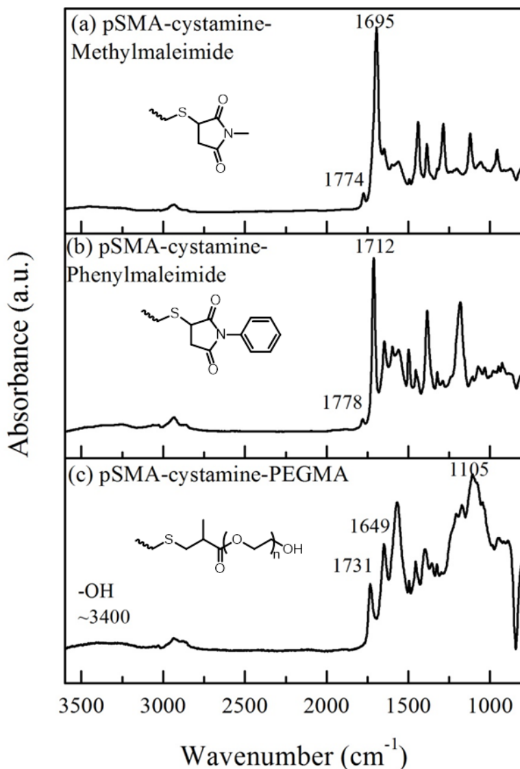
Figure 4.5 gATR-FTIR of (a) N -methylmaleimide, (b) N -phenylmaleimide, (c) poly(ethylene glycol) methacrylate modified reduced pSMA-cystamine polymer brush.
