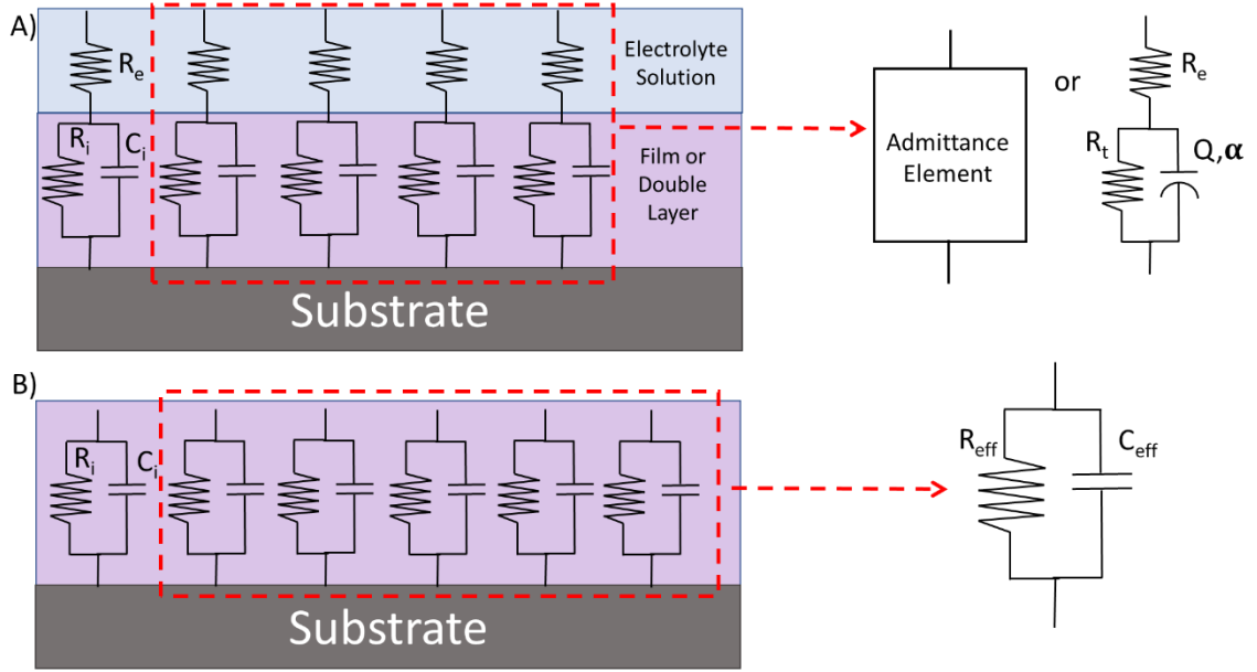
Figure 4.13 Possible circuit diagrams for polymer films based on work from Hirschorn et al. 112
