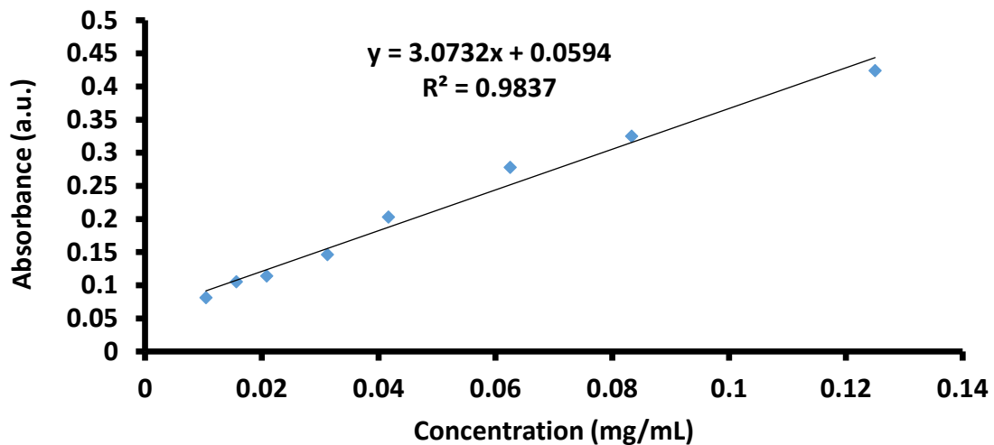
Figure 3.9 UV-Vis absorption calibration curve using dispersed P3HT.
