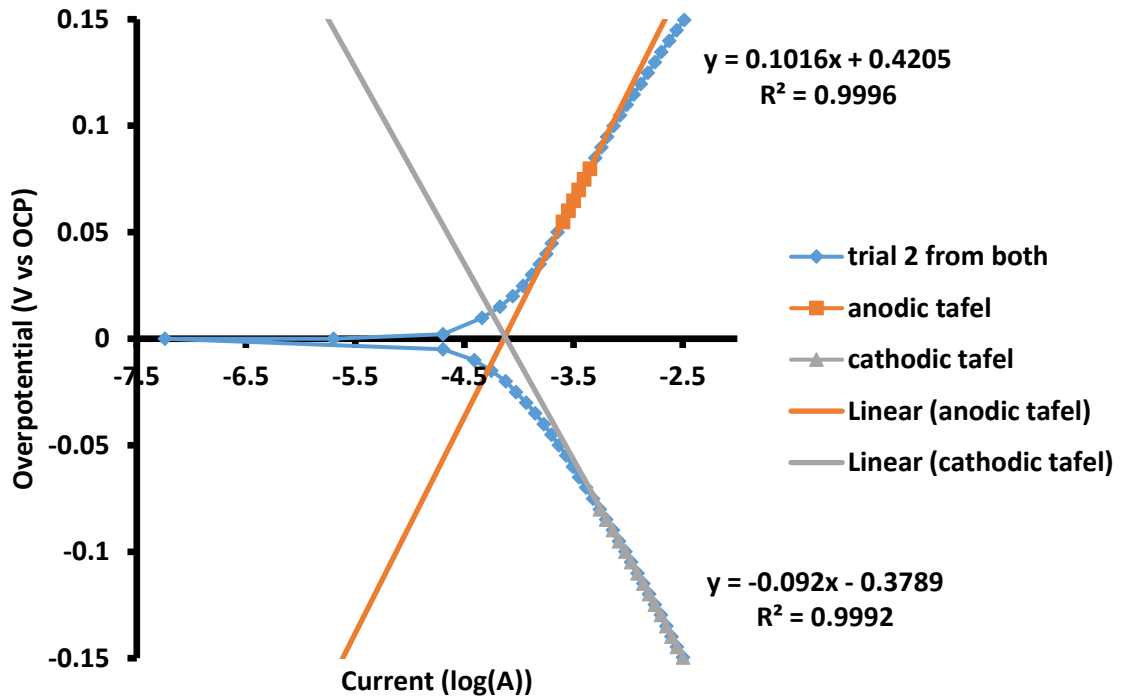
Figure 4.4 Combined anodic and cathodic branches of Tafel plots for steel in 1 M HCl.
