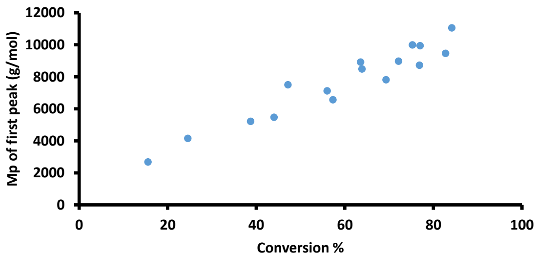
Figure 2.14 Molecular weight vs conversion for P3HT.
