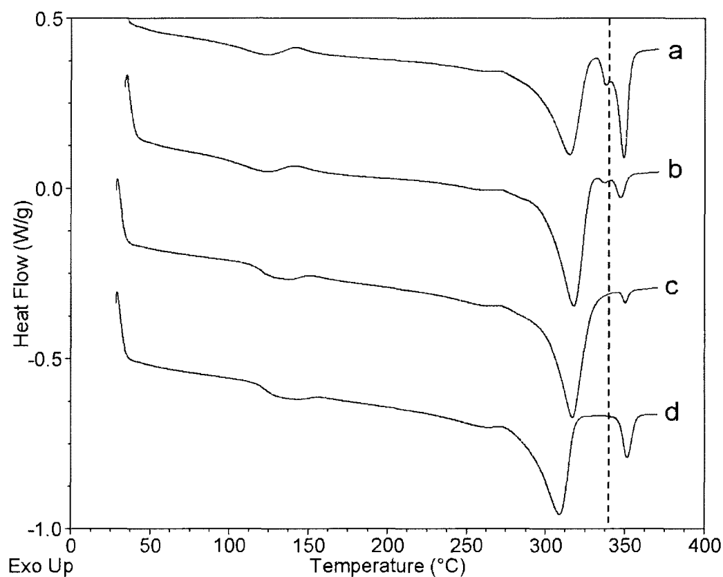
Figure 2.12. DSC thermographs of white (a) and clear (b) regions of compression molded film, and unannealed (c) and annealed (d) non-compression molded samples of the 40:60 wt-% PA-10,T, 6,T copolymer (vertical line represents compression molding and DSC annealing temperature).
