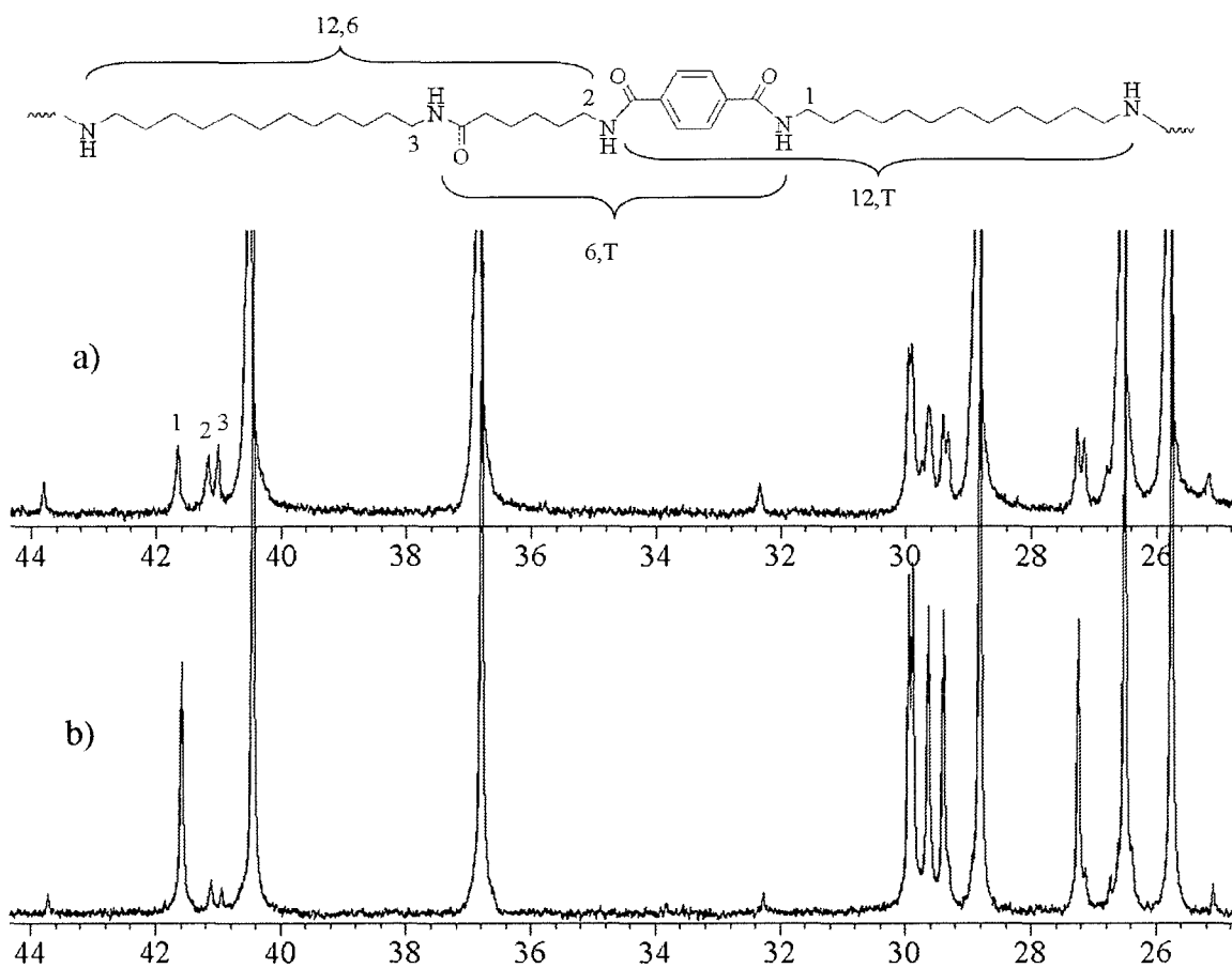
Figure 3.12. 13 C NMR aliphatic regions of the AP of PA-12,T MI with a) 1 and b) 10 mol-% CaCl 2
