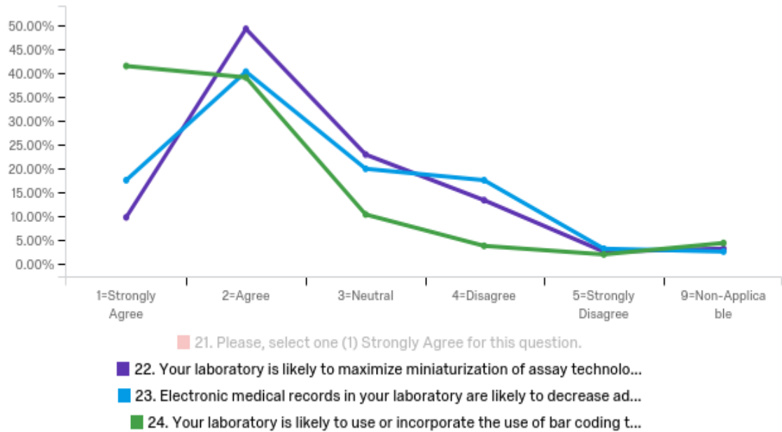
Figure 15. Survey Questions 22-24
