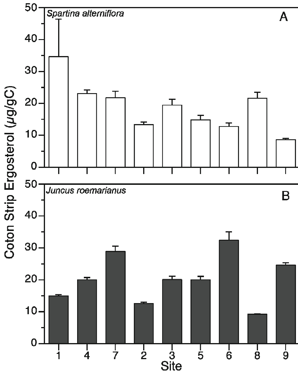
Figure 10. Fungal ergosterol concentrations associated with cotton strips incubated at the marsh surface sediments in the S. alterniflora (A) and J. roemerianus (B) plant zones at each marsh site. Values are the mean \pm SE (n=5)
