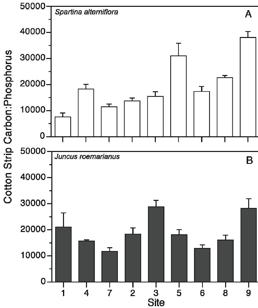
Figure 9. Carbon:phosphorus ratio patterns for cotton strips incubated at the marsh surface sediments in the S. alterniflora (A) and J. roemerianus (B) plant zones at each marsh site. Values are the mean \pm SE (n=5).
