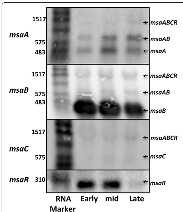
Figure 3 Transcription of the msaABCR operon. Northern blot analyses were performed to detect transcripts produced by the msaABCR operon at three growth phases (early exponential, mid exponential, and late exponential). Gene specific riboprobes were used and are indicated on the left. The identity of the transcripts detected is indicated on the right. Size marker (nt) is shown on the left.
