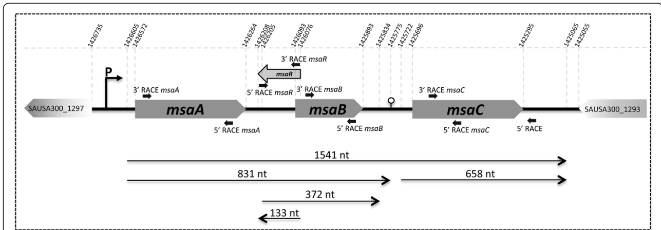
Figure 2 Map of the msaABCR operon. Rapid amplification of cDNA ends (RACE) and Northern blot analyses were used to determine the length and ends (5' and 3') of the RNA transcripts produced by the msaABCR operon. Long thin arrows represent the various RNAs identified in this study, the direction and length in nucleotides (nt) is also indicated. Short thick arrows indicate the positions and directions of the gene-specific primers used in the separate reactions. Reporter gene fusion studies showed the presence of only one active promoter (P) in this operon.
