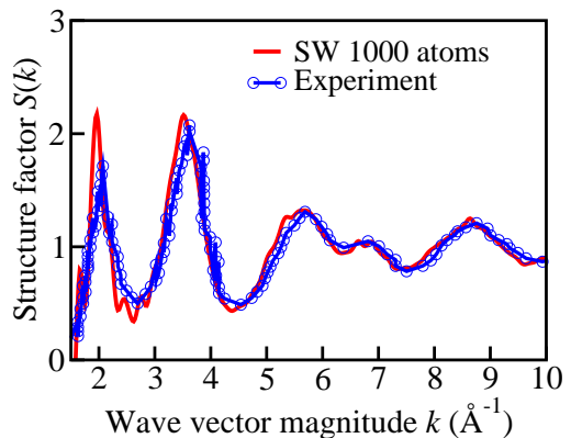
FIG. 3. (Color online) Comparison of the static structure factors of a -Si from molecular-dynamics simulations (SW) and high-energy X-ray diffraction. The experimental data (blue) correspond to annealed samples of a -Si from Laaziri et al. 56
