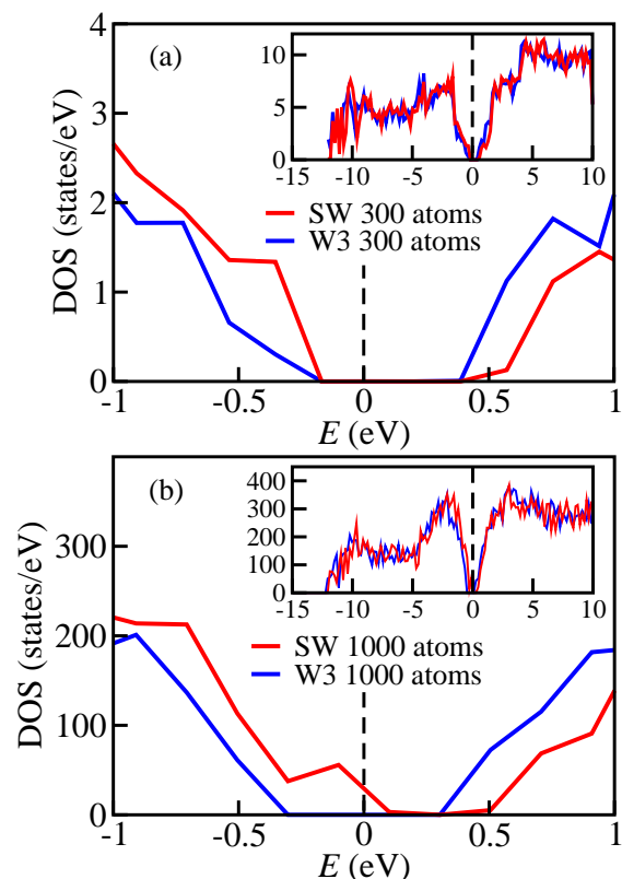
FIG. 7. (Color online) Depiction of the electronic densities of states (EDOS) of a -Si from SW (red) and W3 (blue) models in the regions close to their band-gaps. The full EDOS for the 300- and 1000-atom models are shown as inset in (a) and (b), respectively. The Fermi level is indicated by a dashed vertical line at 0 eV.
