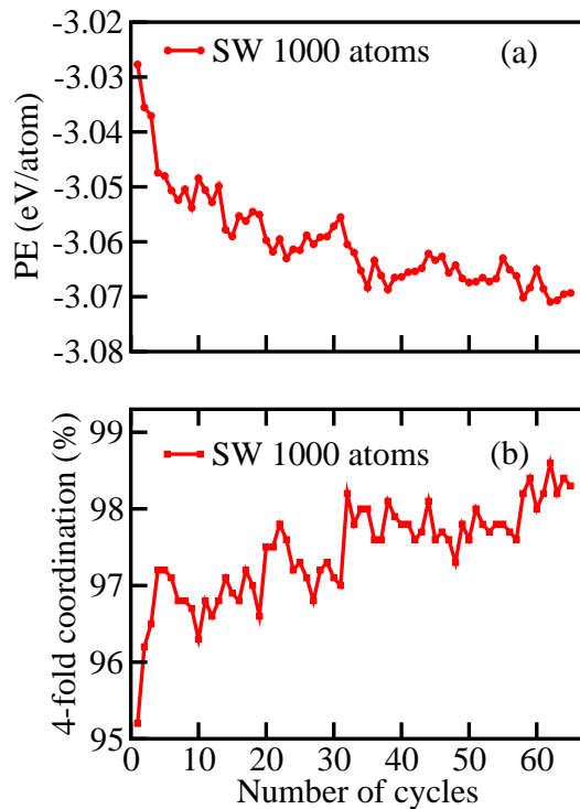
FIG. 1. (a) Time evolution of the potential energy per atom versus number of NVT-NVE cycles. In this illustrative plot, each cycle corresponds to a time period of 300 ps when the simulation temperature decreases from 1800 K to 300 K. (b) Evolution of the number of total atoms (in %) having 4-fold coordination versus the number of NVT-NVE cycles.
