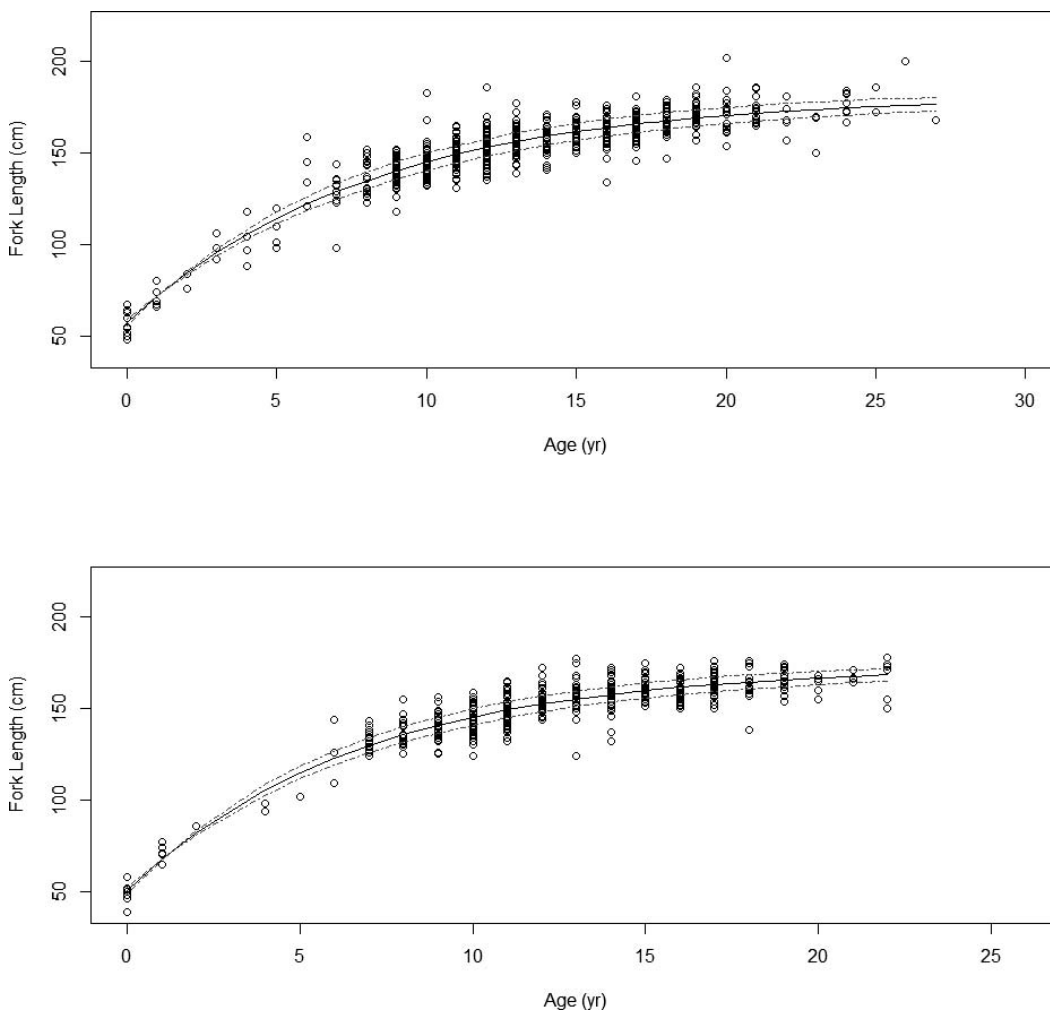
Fig. 5. von Bertalanffy growth curve for (A) male (n = 493, R 2 = 0.88, P < 0.0001) and (B) female sandbar sharks ( Carcharhinus plumbeus ) (n = 701, R 2 = 0.85, P < 0.0001). Model estimates are represented by black solid lines with dashed 95% confidence intervals.
