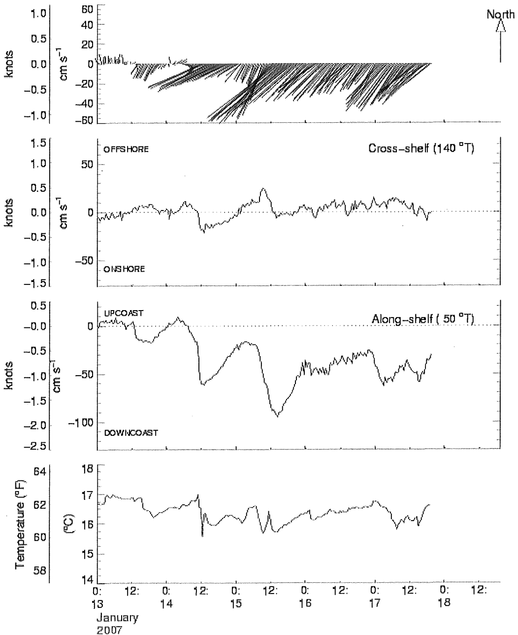
Fig. 5. Level I view of current and water temperature data at buoy H.
