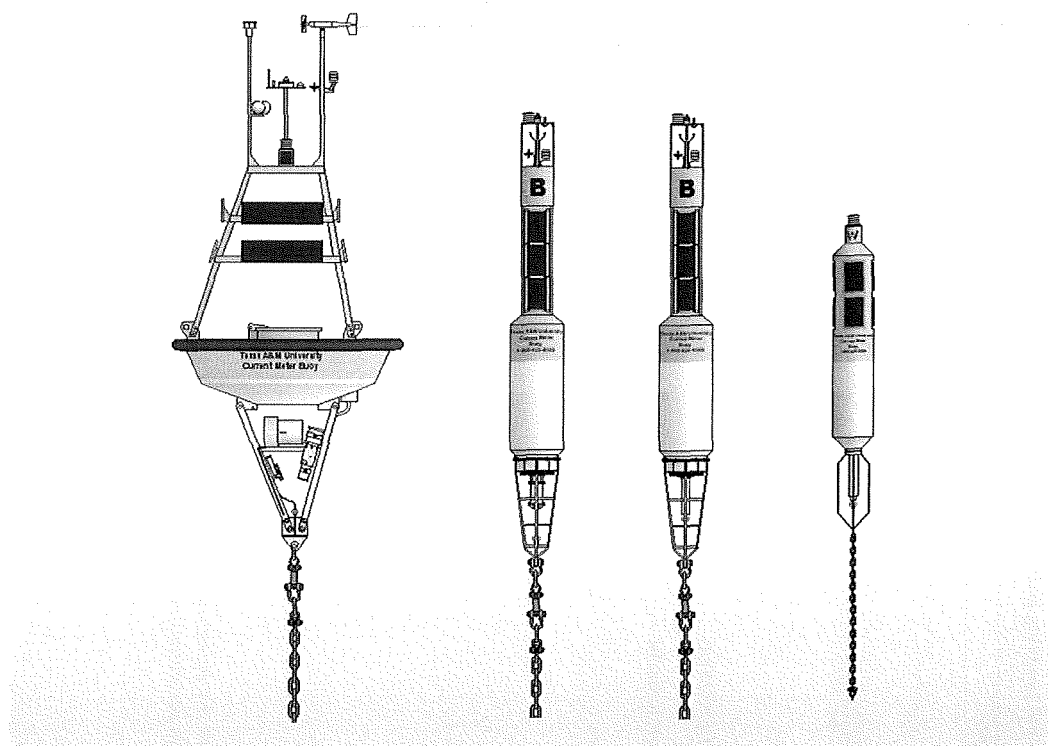
Fig. 2. Schematic of TABS I (far right), TABS II (middle two: leftmost with downward-looking RDI ADCP and Aanderaa DCS 4100R and rightmost with Aanderaa DCS 4100R only) and 3-m discus buoys (far left) fabricated at GERG. The older style Windsonic anemometers are depicted on the two TABS II buoys. Buoys are to scale.
