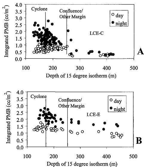
Fig. 5. (A) and (B) Integrated PMB in three different hydrographic regimes during October 1996 and August 1997, respectively. PMB was significantly higher in August 1997 than October 1996, higher at night than in the day, and higher in the cyclone and confluence/other margin areas than in the anticyclones.
