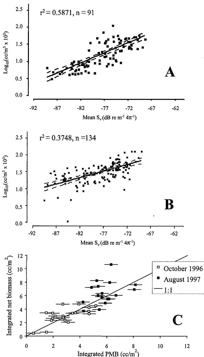
Fig. 3. (A) and (B) Regressions of MOCNESS wet displacement volume biomass on S_v from the ADCP for October 1996 and August 1997, respectively. (C) A comparison of integrated biomass estimates from the MOCNESS and PMB (error bars are 95% prediction intervals).
