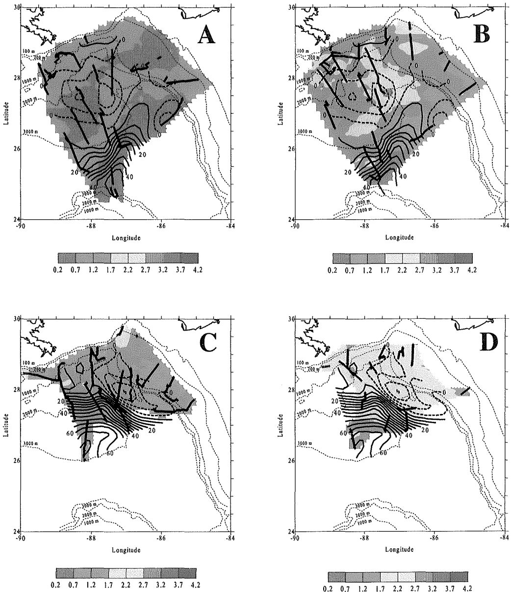
Fig. 4. Gridded and color-contoured distributions of integrated acoustic PMB ( \text{cc}/\text{m}^3 ) for October 1996 (A) day and (B) night and August 1997 (C) day and (D) night. Dynamic height anomaly (0–800 m, dyn cm) is shown by dashed (positive anomaly) and solid (negative anomaly) contour lines. The heavy dark lines indicate locations of integrated PMB data used for contouring.
