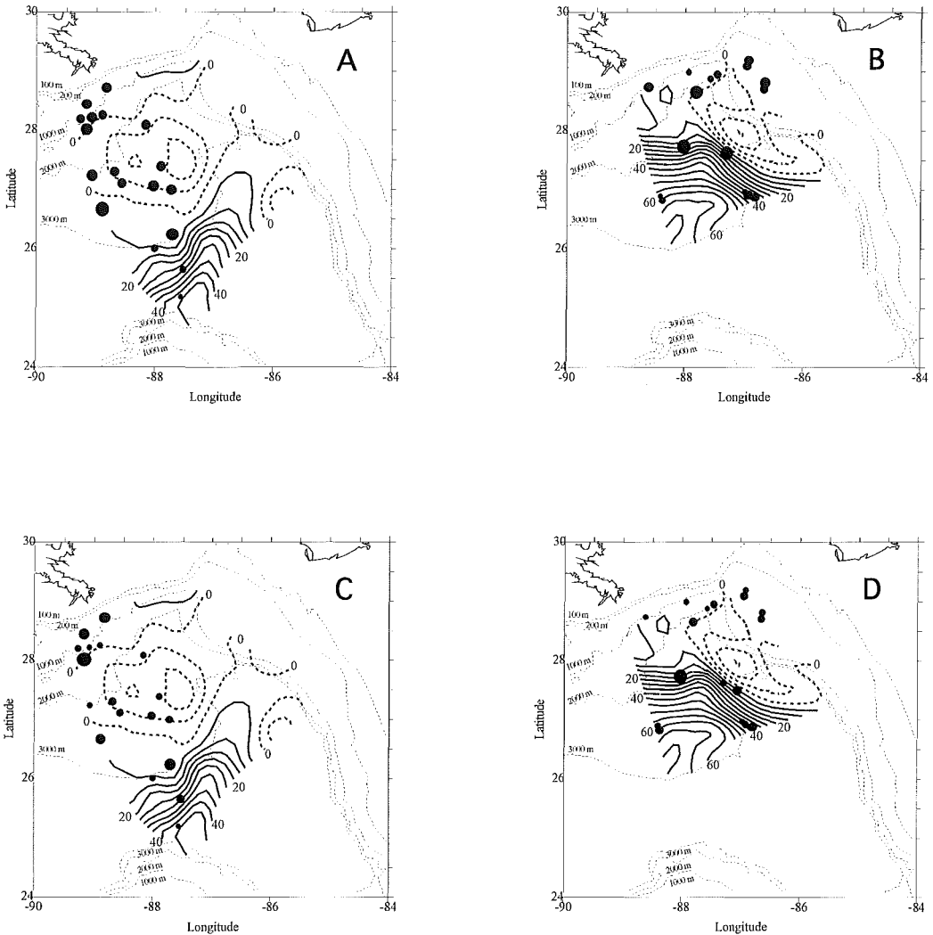
Fig. 1. Integrated zooplankton biomass ( \text{cc}\cdot\text{m}^{-2} ) from 1- \text{m}^2 MOCNESS samples taken during (A) October 1996 and (B) August 1997 and integrated cephalopod paralarval abundance ( \text{no}\cdot\text{m}^{-2} ) from 1- \text{m}^2 MOCNESS samples taken during (C) October 1996 and (D) August 1997. The size of each circle is proportional to the largest value within each plot. Bold solid (positive) and bold dashed (negative) lines are sea surface dynamic height anomaly (DHA, cm) relative to the 100 cm mean. Contour intervals are 5 cm. The cyclone is between 0 and -12 cm, the confluence between 0 and 22 cm, and the anticyclone between 25 and 50 cm.
