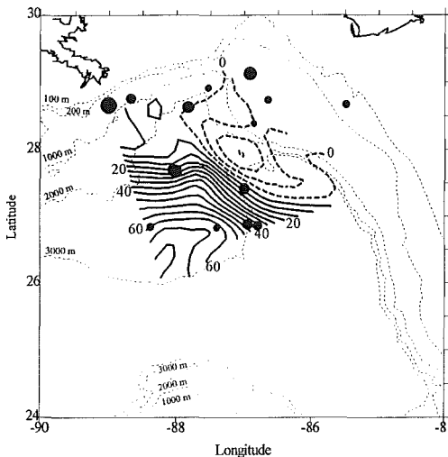
Fig. 2. Integrated myctophid abundance (no.·m -2 ) from the 15-foot Isaacs Kidd midwater trawl tows taken during August 1997. The size of each circle is directly proportional to the largest value within each plot.
