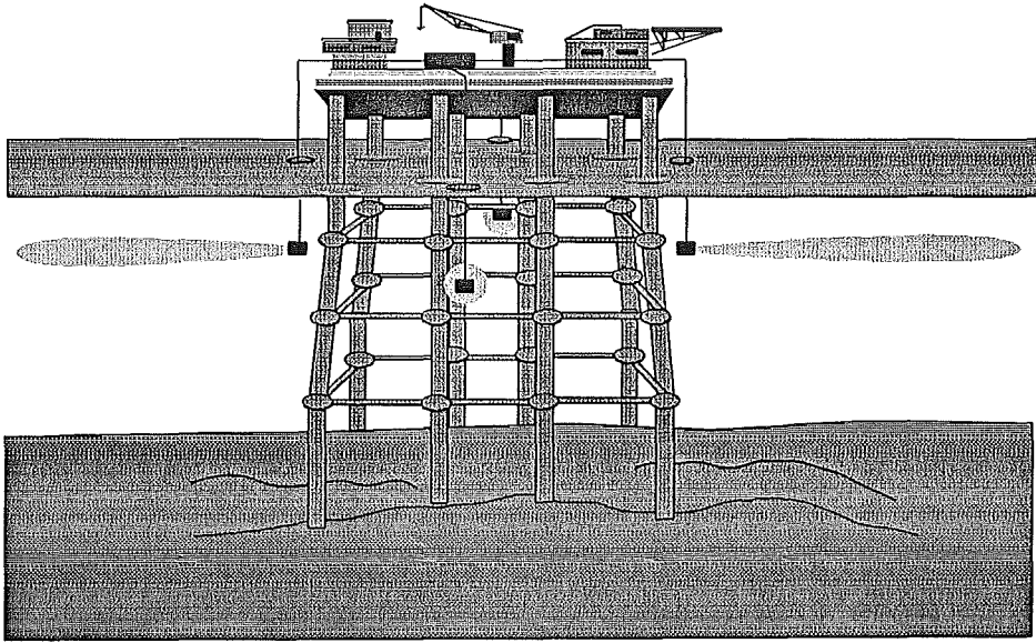
Fig. 1. Schematic view of stationary hydroacoustic transducer deployment to measure horizontal relative density of fishes associated with petroleum platforms.
