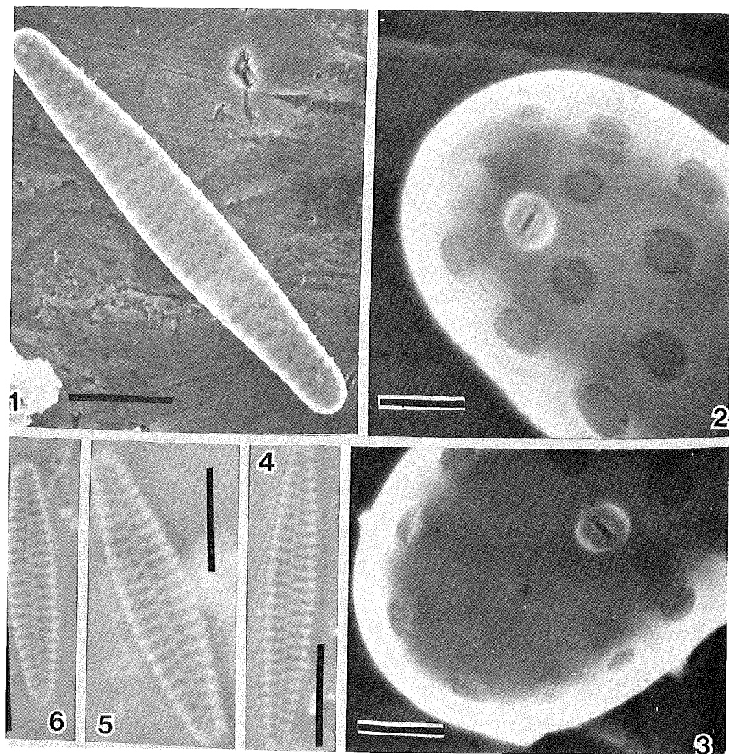
Figure 1. Neodelphineis pelagica Takano from St. George Sound, northeastern Gulf of Mexico. SEM photographs of the interior of the valve. Inset 1-3 show details of valve apices with a single rimoportula, rota type of velum on the areolae, and
