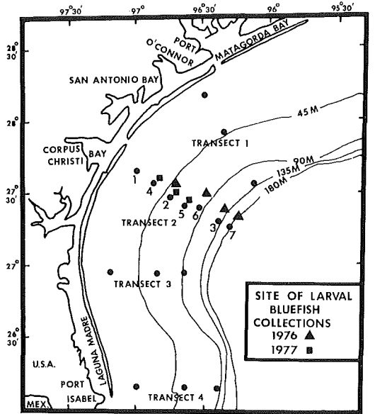
Figure 1. Sampling area off south Texas coast, indicating sites of larval bluefish collections.
