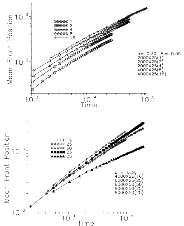
FIG. 1. Mean front position vs time on a log-log scale at a fixed impurity concentration p = 0.30 . Numbers in parentheses are the values of the number of particles N_p . Over 500 independent samples were used for each curve. (a) N_p = 1, 2, 4, 8, and 16 for the forward bias B_{+x} = 0.35 . (b) N_p = 16, 25, and 50 with different lengths L_y = 25 and 50 for the forward bias B_{+x} = 0.35 except the lowest curve, which is with B_{+x} = 0.40 .
