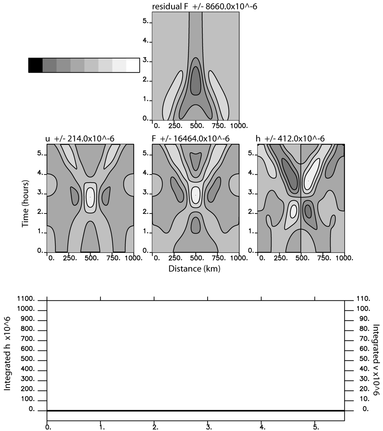
FIG. 4. The representer function for a weak constraint on mass flux and a measurement of velocity indicates (top center) the correction applied to mass flux and how the measurement will affect the solution of (middle left) velocity, (middle center) mass flux, and (middle right) sea level. (bottom) The spatially integrated sea level as a function of time indicates that a velocity measurement conserves mass (solid line) and conserves momentum (dashed line). Shaded areas indicated as in Fig. 2.
