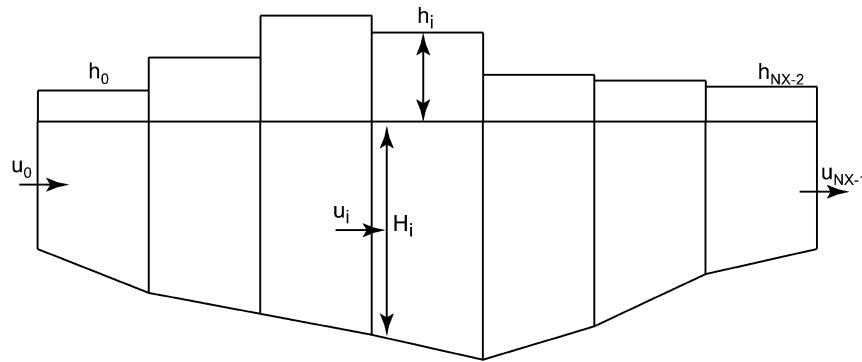
FIG. 1. A one-dimensional C grid is used to represent the dynamical equations. The sea level height \eta exists at points centered between velocity points u . The problem is well posed by specification of the initial conditions for all values of \eta and u along with boundary conditions for u .
