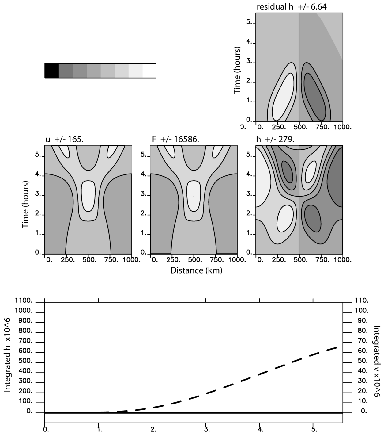
FIG. 2. The representer function for a weak constraint on continuity and a measurement of velocity indicates (top right) the correction applied to continuity and how the measurement will affect the solution of (middle left) velocity, (middle center) mass flux, and (middle right) sea level. (bottom) The spatially integrated sea level as a function of time indicates that a velocity measurement conserves mass (solid line) but does not conserve momentum (dashed line). The numbers above each shaded plot indicate the shade bar range.
