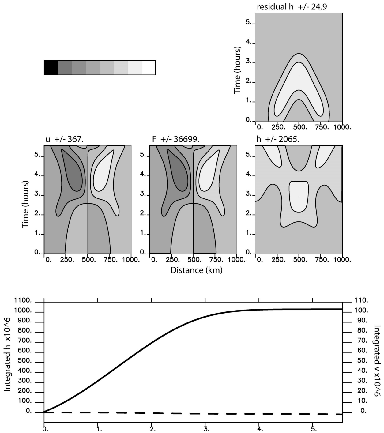
FIG. 3. The same as in Fig. 2 except for a measurement of sea level. (bottom) The spatially integrated sea level as a function of time indicates that a velocity measurement does not conserve mass (solid line) but does conserve momentum (dashed line). Shaded areas indicated as in Fig. 2.
